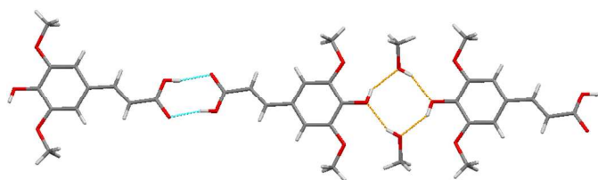
Figure 6. The reported crystal structure of the methanol solvate of sinapic acid (WAMFOG). 32
