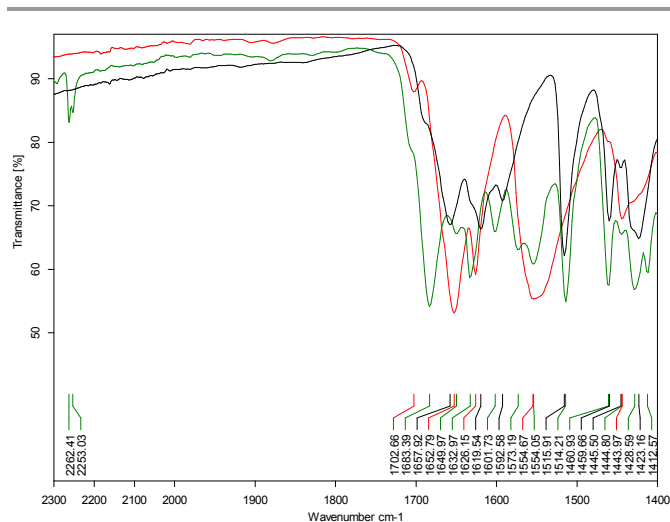
Figure 4. Expanded view of the IR spectrum of SA.PTU.2MeCN showing the region from 1400-2300 \text{cm}^{-1} (black – SA ; red – PTU ; green – SA.PTU.2MeCN ).
