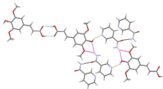
Figure 7. A section of the crystal structure of SA.NIA highlighting the key hydrogen bonding interactions.
