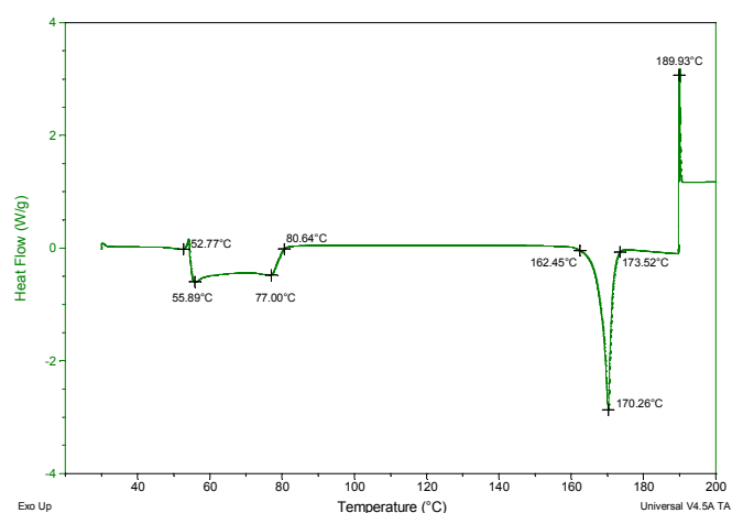
Figure 12. DSC spectrum of SA.PTU.2MeCN showing the loss of the acetonitrile molecules.
