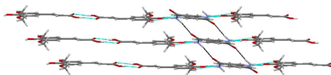
Figure 8. Amide N-H...O=C amide C(4) chains (black) responsible for interlinking adjacent layers in the SA.NIA co-crystal.
