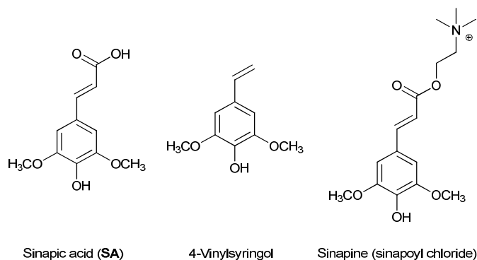
Figure 1. Structure of sinapic acid and its bioactive derivatives.
