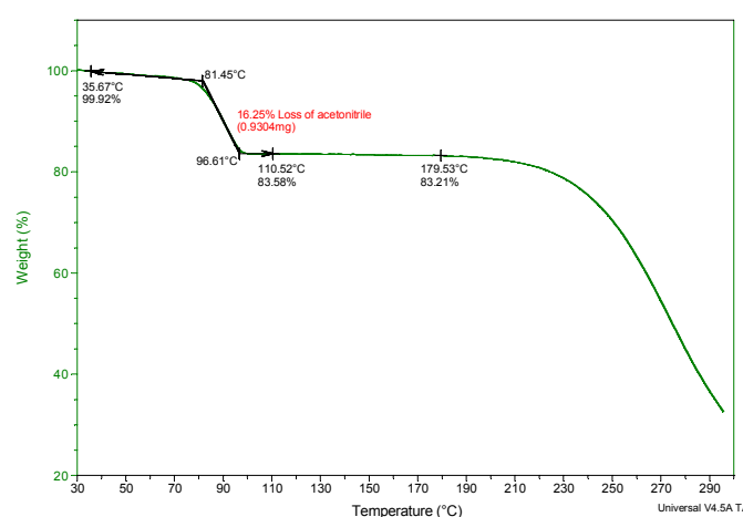
Figure 13. TGA spectrum of SA.PTU.2MeCN showing the loss of the acetonitrile molecules.
