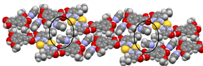
Figure 11. Space-filling model of the crystal structure of SA.PTU.2MeCN highlighting the voids occupied by acetonitrile molecules.
