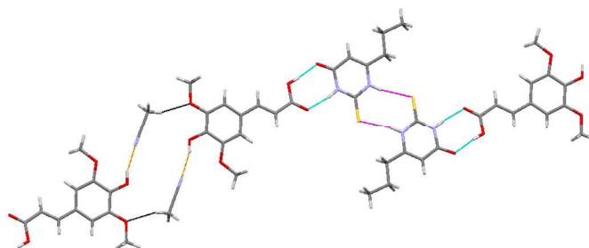
Figure 10. A section of the crystal structure of SA.PTU.2MeCN highlighting the key hydrogen bonding interactions.
