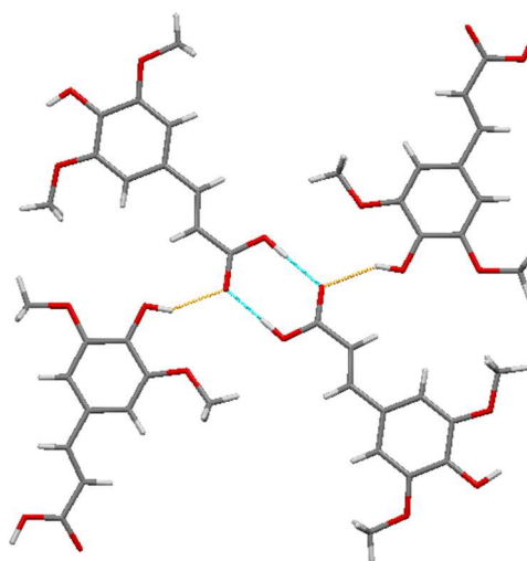
Figure 5. A section of the crystal structure of SA highlighting the key hydrogen bonding interactions.
