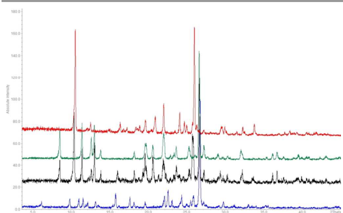
Figure 14. PXRD pattern of SA.PTU.2MeCN (blue) compared with desolvated sample (black), sinapic acid (green), and 6-propyl-2-thiouracil (red).
