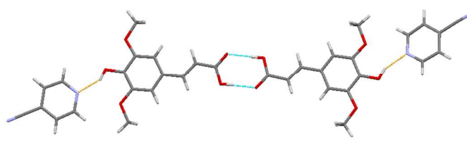
Figure 9. A section of the crystal structure of SA.PYC highlighting the key hydrogen bonding interactions.
