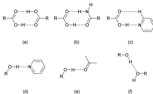
Figure 2. Common hydrogen-bonding motifs involving acids (a-c) and phenols (d-f).
