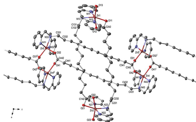
Fig. 12 ORTEP diagram of the \text{Zn}^{\text{II}} macrocycle and polymer 9 . All hydrogen atoms, perchlorate anions and solvent have been omitted for clarity. For bond lengths, angles and coordination geometries see Table S5†. Symmetry codes: (i) x, 1 - y, 1/2 + z ; (ii) x, 1 - y, z - 1/2 .
