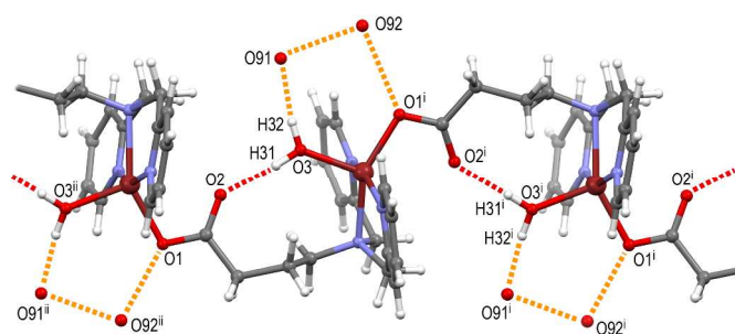
Fig. 3 Detail of hydrogen bonding interactions for 1 . Intramolecular H-bonding interactions are shown in red and intermolecular interactions in orange; \text{O3} \cdots \text{O2} 2.683(3), \text{O3} \cdots \text{O91} 2.703(8), \text{O91} \cdots \text{O92} 2.649(8), \text{O92} \cdots \text{O1}^i 2.823(5) Å. Symmetry codes: (i) 1/2 + x, 1/2 - y, 1/2 + z ; (ii) -1/2 + x, 1/2 - y, -1/2 + z .
