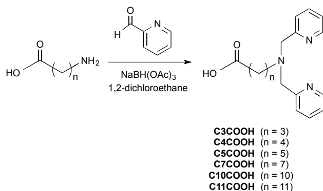
Scheme 1 General synthesis of di(2-pyridylmethyl)alkylamine-appended carboxylate ligands C n COOH .
