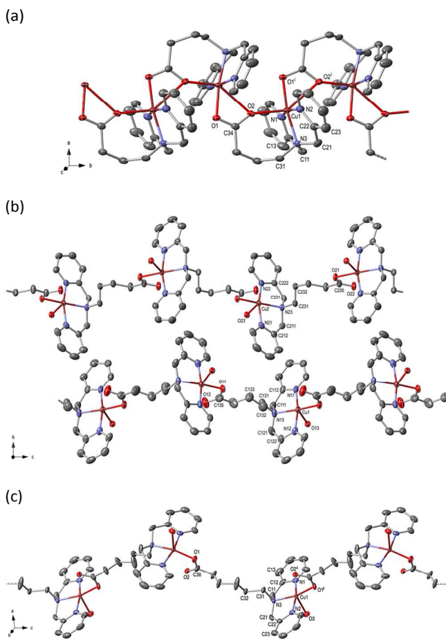
Fig. 4 ORTEP diagrams of the Cu II coordination polymers (a) 4, (b) 5, and (c) 6. All hydrogen atoms, perchlorate anions and solvent have been omitted for clarity. For bond lengths, angles and coordination geometries see Table S4†. Symmetry codes: (i) 3/2 – x, 1/2 + y, 1/2 – z; (ii) 1 – x, 1/2 – y, 1/2 + z.
