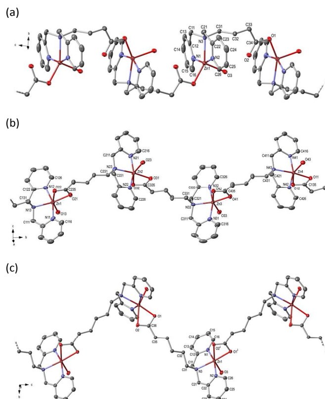
Fig. 2 ORTEP diagrams of the \text{Zn}^{\text{II}} coordination polymers (a) 1 ( n = 3 ), (b) 2 , ( n = 4 ), and (c) 3 ( n = 5 ). All hydrogen atoms, perchlorate anions and solvent have been omitted for clarity. For bond lengths, angles and coordination geometries see Table S3†. Symmetry code: (i) x, 1/2 - y, 1/2 + z .
