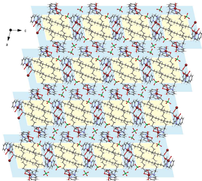
Fig. 15 Packing diagram of the Zn II macrocycle and polymer 9 viewed down the b -axis showing the nanosegregation of the aromatic (blue highlight) and aliphatic (yellow highlight) components of the ligands, extending into the page along the b -axis. The second component of the disordered perchlorate anions and lattice water have been omitted for clarity.
