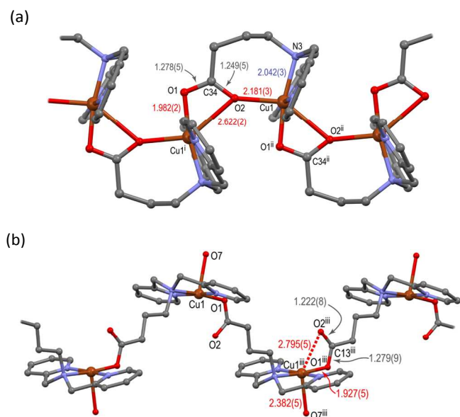
Fig. 5 Detail of the bonding of the carboxylate groups of (a) 4 ( n = 3 ) and (b) a related Cu(II) structure of the same ligand (CSD code: EYEHAR). 8c Hydrogen atoms, perchlorate anions and solvent molecules omitted for clarity. Symmetry codes: (i) 3/2 - x, -1/2 + y, 1/2 - z ; (ii) 3/2 - x, 1/2 + y, 1/2 - z ; (iii) 3/2 - x, -1/2 + y, 1/2 + z .
