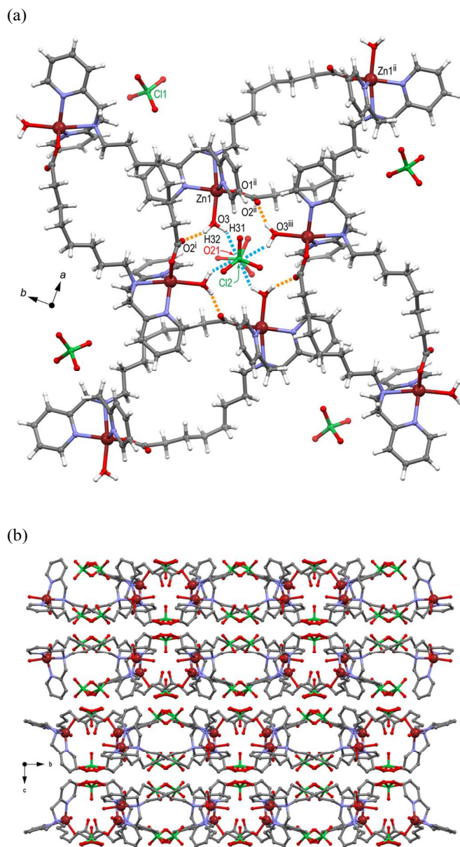
Fig. 7 Packing diagram of the Zn II macrocycle 7 ( n = 7) (a) viewed down the c -axis. Intermolecular H-bonding interactions at the inversion centre involve the aqua ligand hydrogens and a neighbouring carboxylate carbonyl oxygen (O3–H32...O2' 1.79(6), O3...O2' 2.597(6) Å; dashed orange lines) and perchlorate oxygen (O3–H31...O21 2.26(6), O3...O21 2.964(2) Å; dashed blue lines), (b) viewed down the a -axis showing the layered structure. Disordered perchlorate anions are shown in all possible sites. Symmetry codes: (i) y - 1/4, 5/2 - x, 1/4 - z ; (ii) 1 - x, 1/2 - y, z ; (iii) y - 1/4, 1/4 - x, 1/4 - z .
