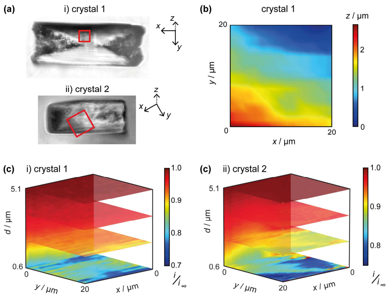
Fig. 5. (a) Bright field optical microscopy images of i) crystal 1 and ii) crystal 2, taken after HIC-SECM. The 20 \times 20 \mu\text{m} scan area is represented by the red square. (b) Topography of crystal 1 with the lowest point of the crystal imaged designated as z = 0 . (c) 3D plots of the normalised tip current ( i/i_\infty ), revealed above crystals 1 and 2, with several horizontal and vertical slices through the data sets highlighted.
