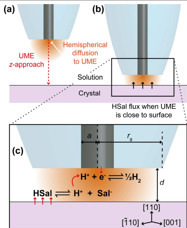
Fig. 1. Schematic showing a UME in bulk solution, at a sufficient distance from the crystal that HSal/H + reduction does not induce HSal dissolution (a) and close to the crystal such that the surface dissolves due to local undersaturation between the tip and crystal, induced by the UME process (b). (c) Zoom-in of part (b) showing the reactions occurring on the (110) face of salicylic acid and the UME. The reduction of protons at the UME surface causes the dissociation of salicylic acid through local undersaturation. When the UME is brought close to the salicylic acid crystal, this localised undersaturation causes the crystal surface to dissolve to replenish aqueous salicylic acid and is manifested as a higher current at the UME, than would be expected for an inert surface with the UME at the same distance. Note that this diagram is not to scale.
