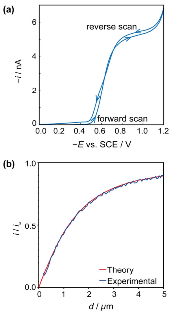
Fig. 4. (a) Typical cyclic voltammogram for the reduction of HSal (via dissociation to \text{H}^+ and \text{Sal}^- ) at a 2.5 \mu\text{m} diameter Pt UME. (b) Tip approach curves (applied potential -0.8 \text{ V} ) to an insulating (glass) surface with the same UME. The blue approach curve is the experimental data, and red curve is the theoretical result for hindered diffusion for an electrode with RG = 15 . 44
