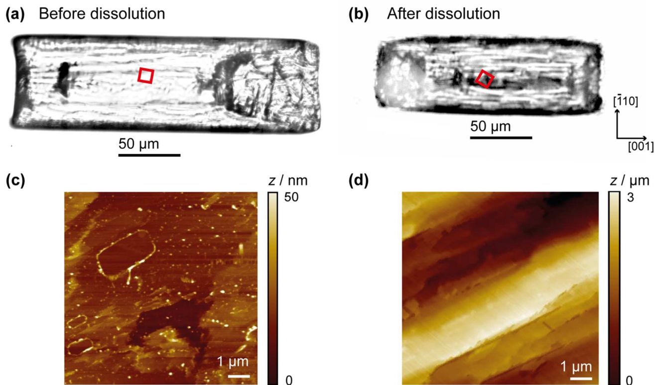
Fig. 7. Bright field optical microscopy images of a salicylic acid crystal, not imaged by HIC-SECM, (a) before dissolution (as-grown) and (b) after 15 mins dissolution in an 8.4 mM solution of salicylic acid. The 9 \times 9 \mu\text{m} scan area is represented by the red square. (c) Ex-situ AFM topography images of the crystals in (a) and (b) are shown in (c) and (d), respectively. Note the difference in height scale bars.
