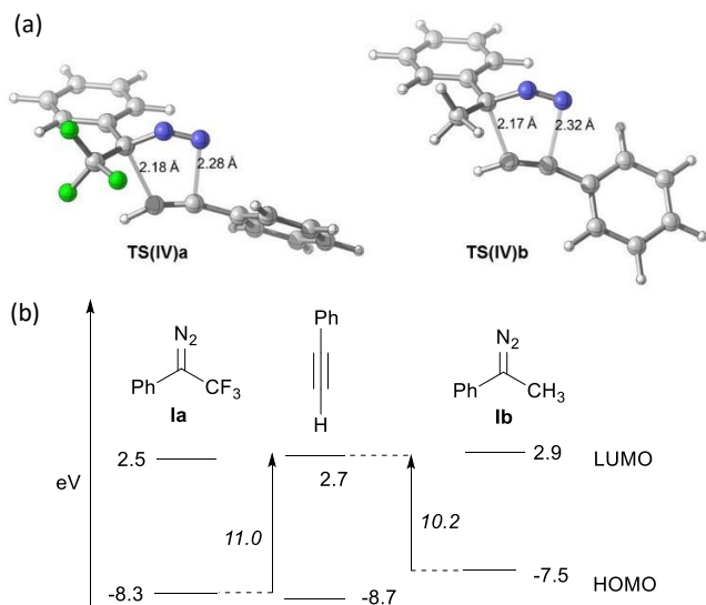
Figure 2: Figure 2. (a) Transition structures TS(IV) obtained for the 1,3-dipolar cycloadditions of phenylacetylene with the 1-(dialzo-2,2,2-trifluoroethyl)benzene la and 1-dialzoethylbenzene lb respectively obtained at the M06-2X/6-311++G** level. (b) Representation of the energies of the Frontier Orbitals responsible for the main interactions in the 1,3-dipolar cycloaddition. Frontier Orbital Energies (eV) have been obtained from a single point HF/6-311G** calculation on the geometries optimized at the M06-2X/6-311++G** level.
