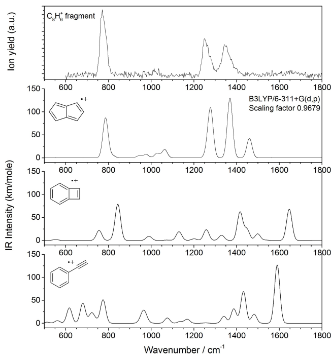
Fig. 3 Infrared photo-dissociation spectrum of C_8H_6^+ formed from the dissociative ionization of naphthalene (top) shown together with the computed spectra of the C_8H_6^+ isomers pentalene, benzocyclobutadiene and phenylacetylene.
