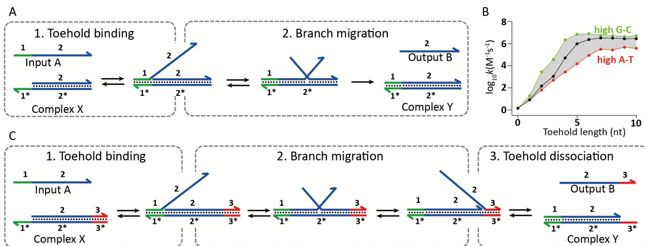
Fig. 3 Underlying mechanisms used in dynamic DNA circuits. (A) Schematic representation of the toe-hold-mediated strand displacement reaction. Input A binds to the toe-hold-sequence 1* present on complex X, initiating subsequent branch migration. Completion of branch migration results in the release of output B and the formation of complex Y. Since the resulting complex Y has no available toe-hold, the reverse reaction is effectively not taking place. (B) The rate of toe-hold-mediated strand displacement is highly dependent on the length and sequence of the toe-hold domain. Increasing the stability of the toe-hold results in an enhanced displacement rate (adapted with permission from ref. 21, copyright 2009, American Chemical Society). (C) Schematic representation of the toe-hold-exchange mechanism. Input A binds to the toe-hold-sequence 1* present on complex X, initiating subsequent branch migration. After branch migration output B is bound to the complex via toe-hold-sequence 3*, which has to spontaneously dissociate for the toe-hold exchange reaction to complete, resulting in the release of output B and the formation of complex Y. Since complex Y contains a toe-hold-sequence to which output B can bind, the reverse reaction can also take place.
