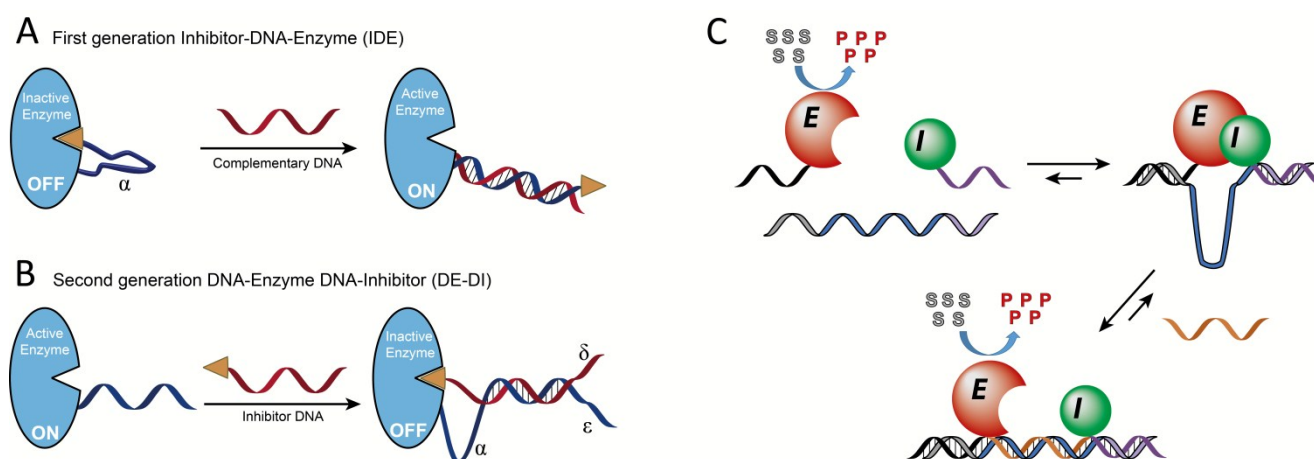
Fig. 7 Mechanical control of enzyme-inhibitor complex formation. (A) First generation Inhibitor-DNA-Enzyme (IDE) system. A small-molecule phosphoramidite inhibitor is conjugated to the Cereus neutral protease enzyme via a ssDNA tether, allowing the inhibitor to bind to the enzyme intramolecularly. Hybridization to the complementary target DNA forces the inhibitor away from the enzyme (adapted with permission from ref. 48, copyright 2003, American Chemical Society). (B) Second generation DNA-enzyme-DNA-inhibitor (DE-DI) system. Hybridization of a DNA strand functionalized with a small-molecule inhibitor to an enzyme-DNA chimera. Multiple single-stranded regions ( \alpha , \delta and \epsilon ) allow more complex operations like OR, NOR and AND Boolean logic gates. Figure adapted from ref. 49, copyright 2007, John Wiley and Sons. (C) Non-covalent formation of an enzyme-inhibitor complex via DNA tethers conjugated to both proteins. Due to their low intrinsic affinity TEM1- \beta -lactamase and the inhibitor protein BLIP only form an inactive complex upon binding to a template oligonucleotide that is complementary to both tethers. Enzyme-inhibitor complexation leads to the formation of a single stranded target recognition loop in the template strand. Binding of the complementary target oligonucleotide to this loop results in the disruption of the enzyme-inhibitor complex, reactivating enzyme activity (reprinted with permission from ref. 50, copyright 2015, American Chemical Society).
