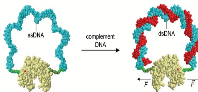
Fig. 6 A mechano-sensitive enzyme actuated by a “DNA spring”. A 60 nucleotide long ssDNA linker is conjugated with both ends to the two lobes of guanylate kinase. By binding of the complementary oligonucleotide, the mechanical properties of the DNA linker change, transforming it into a rigid rod. The rigidity of the linker exerts a mechanical force on the protein, reducing its catalytic activity. Figure adapted from ref. 46. Copyright (2009), with permission from Elsevier.
