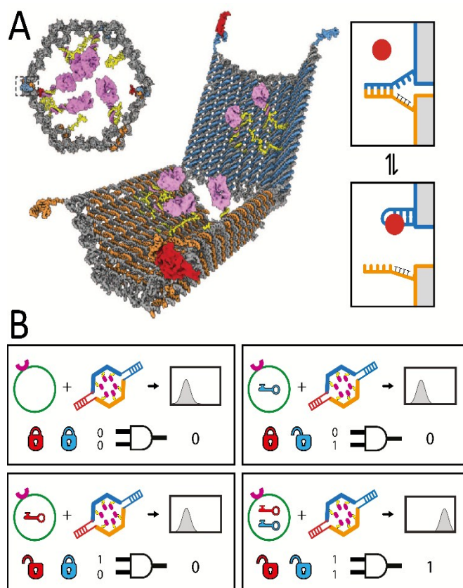
Fig. 12 Autonomous cell surface evaluation by a DNA nanorobot carrying a single chain antibody fragment payload. (A) The hexagonal barrel is loaded with antibody fragments towards human leukocyte antigen and closed by two aptamer based locks, refraining the antibody fragments from binding to the cell surface target. (B) Only in the presence of the right combination of protein inputs the aptamer locks change conformation and allow the barrel to open. Consequently the encapsulated antibodies are able to bind to the cell surface. Figure adapted from ref. 27. Reprinted with permission from AAAS
