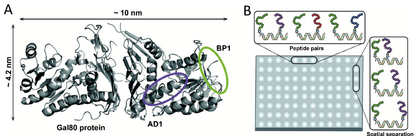
Fig. 9 DNA as a scaffold for multivalent ligand display and subsequent strong protein binding. (A) As a proof of principle a synbody was created that binds multiple, non-overlapping regions of the yeast regulatory protein Gal80. (B) Combinatorial screening of multiple peptide ligands, as well as linker lengths and orientations on a high throughput surface plasmon resonance (SPR) chip allows easy screening for optimal peptide combination and inter-peptide distance (reprinted with permission from ref. 61, copyright 2009, American Chemical Society).
