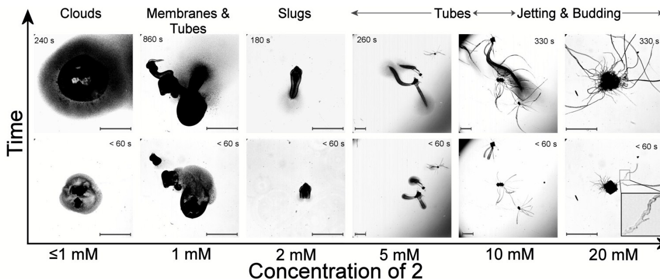
Figure 3 The range of precipitation structures observed for the polyoxometalate-polyoxocation system described here, ranging from cloud like structures at low concentrations to jetting and budding tubes at higher concentrations. Inset on lower 20 mM figure highlights the budding growth regime. Scale bars = 400 \mu\text{m} .
