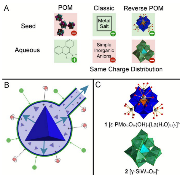
Figure 1 A – A graphical representation of some different types of chemical gardens that are known; previously reported POM based chemical gardens, classic chemical gardens and the charge reversed POM chemical gardens presented herein. B – schematic representation of the general POM chemical garden growth mechanism. C – Structures of the POMs used in the study. Blue – Mo, Orange – P, Grey – La, Red – O, Green – W, Teal – Si.
