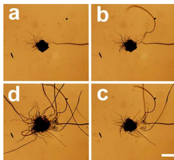
Figure 2 Photos from SV6 showing tube growth at 20 mM after 10 (a), 40(b), 70(c) and 220 (d) seconds. Scale bar is 200 \mu\text{m} .
