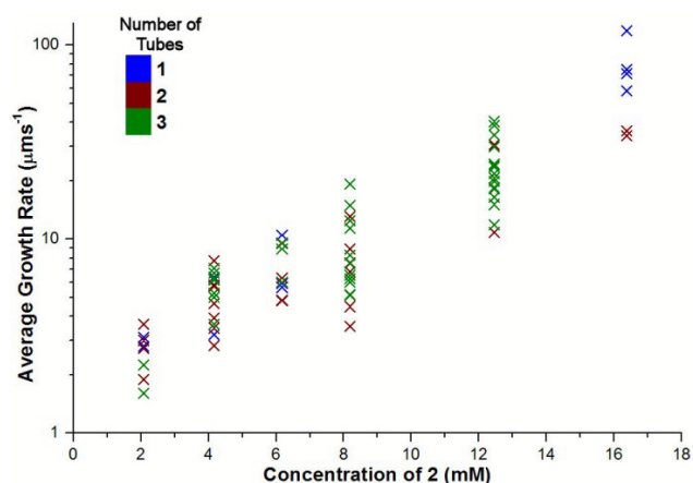
Figure 5 A plot showing the exponential trend between the anion (2) concentration and the tube growth rate.
