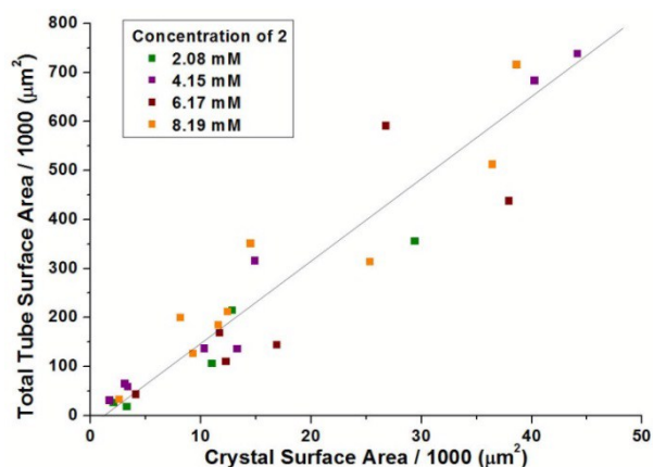
Figure 4 A plot showing the linear correlation between the crystal surface area and the tube surface area formed, when measured from above. Guideline to illustrate trend only.
