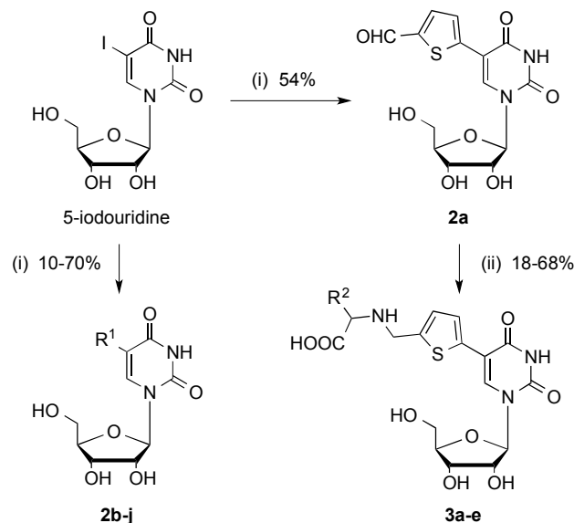
Scheme 1 Synthesis of uridine derivatives 2 and 3 . Reagents and conditions: (i) boronic acid, Pd catalyst, ligand, base, solvents, microwave irradiation; (ii) amino acids, NaBH_3CN , MeOH, rt, 1d. For details and individual yields see ESI, for R^1 / R^2 see Table 1.
