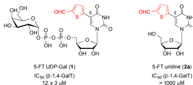
Figure 1 Prototype GalT inhibitor 1 , and the corresponding nucleoside derivative 2a .
