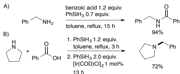
Scheme 3. a) Direct amidation reaction. b) Proof of concept of a one-pot two-step reductive alkylation reaction from carboxylic acids.
