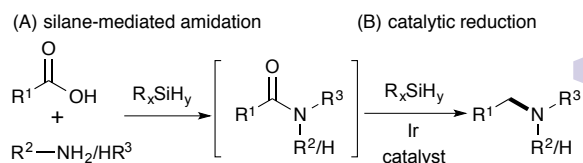
Scheme 2. Catalytic N -alkylation of amines based upon silane dual reactivity.
