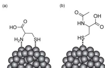
Figure 2. (a) Schematic of cysteine coordination to a platinum particle. (b) Schematic of acetylcysteine coordination to a platinum particle. Due to a higher amount of coordination in Cys@Pt, less randomization process of the para-spin state of hydrogen on the particles surface can occur, leading to higher polarization.
