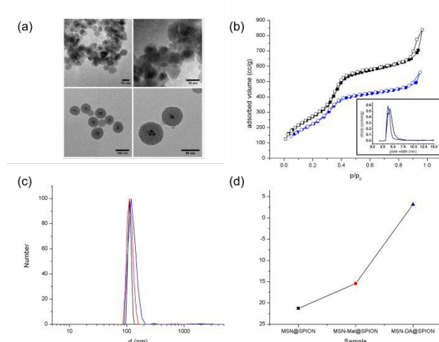
Fig. 2: (a) TEM images of zinc and manganese doped iron oxide nanoparticles ( Zn_{0.4}Mn_{0.6}Fe_2O_4 ; top) and SPION@MSN (bottom) at different magnifications; (b) nitrogen adsorption (filled symbols) and desorption (open symbols) isotherms of sample SPION@MSN (black squares) and SPION@MSN-DA (blue circles) (inset: NLDFT pore size distribution); (c) dynamic light scattering of samples SPION@MSN (black), SPION@MSN-Mal (red) and SPION@MSN-DA (blue); (d) zeta potential analysis at pH=7 of samples SPION@MSN (black square), SPION@MSN-Mal (red circle) and SPION@MSN-DA (blue triangle; the line is a guide to the eye).
