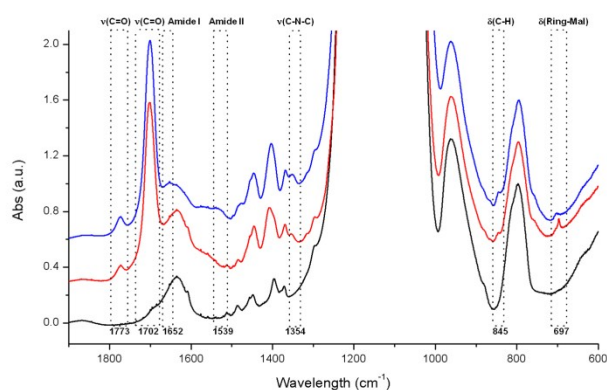
Fig. 3: IR data for samples SPION@MSN (black), SPION@MSN-Mal (red), and SPION@MSN-DA (blue). The vibrations discussed in the text are highlighted by boxes. Peak assignments are based on literature data. 37 For further information and raw spectral data see Fig. S2 in the supplementary information.
