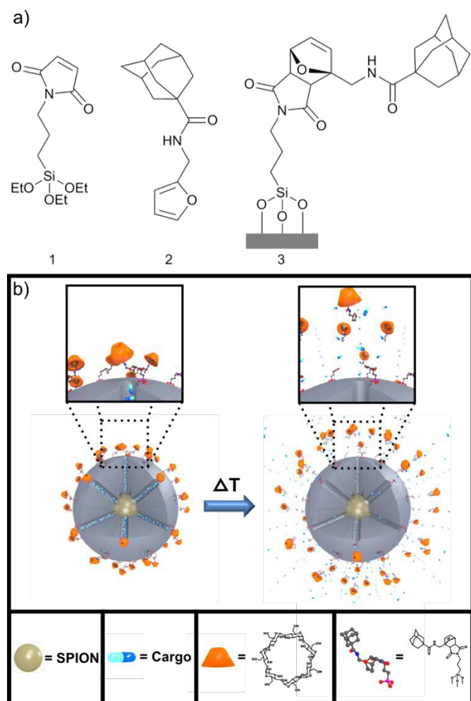
Fig. 1: (a) Chemical structures of the dienophile (1), the diene (2) and the Diels-Alder cycloaddition product (3). (b) Schematic representation of the operating principle of the thermoresponsive nanovalve. A change in temperature triggers a cycloreversion reaction which leads to a dissociation of the bulky gatekeepers from the silica surface and allows cargo molecules to diffuse out of the mesopores.
