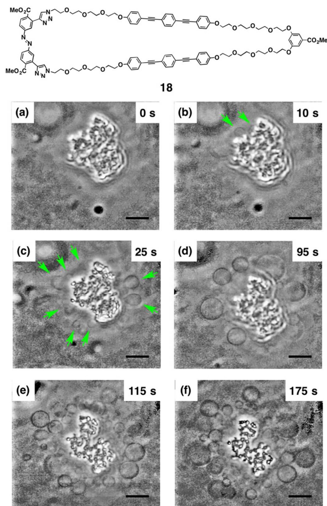
Fig. 13 Molecular structure of 18 . Time-course phase-contrast microscopic observation of the light-triggered \mu -size vesicle formation from a shapeless particle composed of DOPC and 18 in an aqueous solution of glucose and sucrose ([DOPC] = 200 \mu M, [ 1 ] = 40 \mu M, [glucose] = [sucrose] = 100 mM). Snapshots were taken after irradiation (330–385 nm) at 20 °C for (a) 0, (b) 10, (c) 25, (d) 95, (e) 115, and (f) 175 s, respectively. The yellow arrows indicate the generated \mu -size vesicles. The scale bars, 10 \mu m. Reference: 75.
