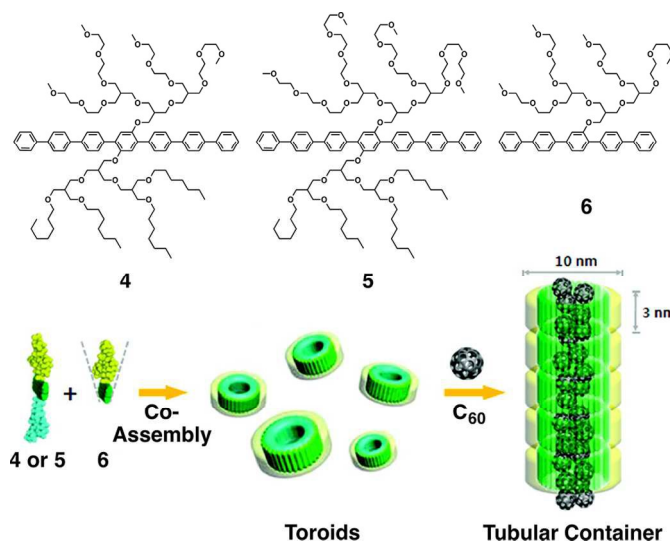
Fig. 5 Laterally grafted multi-block amphiphiles 4 , 5 and 6 . Schematic illustration of co-assembly of 4 or 5 and 6 into toroids and C_{60} -triggered formation of tubular containers. Copyright 2009 from American Chemical Society. Reference: 41.
