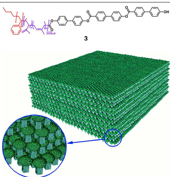
Fig. 4 Multi-block rod-coil molecule 3 forming mushroom-shaped assemblies that organizes into a macroscopic film with asymmetric surfaces. Copyright 1997 from AAAS. Reference: 27.
