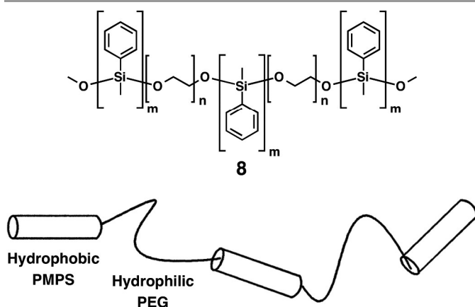
Fig. 7 Molecular structure of (AB) n -type multiblock copolymer 8 and its schematic drawing. Copyright 2000 from American Chemical Society. Reference: 47.
