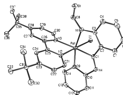
Figure 1. Ortep drawing (50% probability ellipsoids) of complex 4 ·CH 2 Cl 2 .
