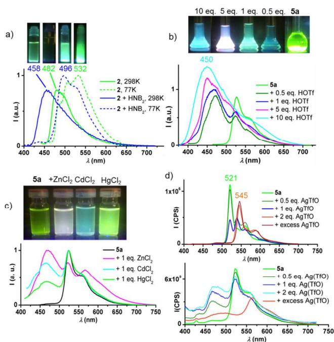
Fig. 1. (a) PL of 2 ( \text{CH}_2\text{Cl}_2 , 1 \times 10^{-4} M) in the absence and presence of two equivalents of [\text{H}(\text{OEt}_2)_2][\text{H}_2\text{N}\{\text{B}(\text{C}_6\text{F}_5)_3\}_2] (HNB 2 ) at 298 and 77 K. (b) PL response of 5a ( \text{CH}_2\text{Cl}_2 , 1 \times 10^{-4} M) to the addition of HOTf at 298 K. (c) PL of mixtures of 5a ( \text{CH}_2\text{Cl}_2 , 1 \times 10^{-4} M) to the addition of \text{MCl}_2 ( \text{M} = \text{Zn}, \text{Cd}, \text{Hg} ) in THFMe-2 ( [\text{5a}] = 10^{-4} M) at 298 K. (d) PL response of 5a (THFMe-2, 5 \times 10^{-4} M) to the addition of \text{AgTfO} at 298 and 77 K.
