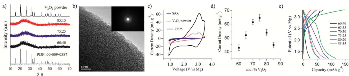
Fig. 1 a) XRD patterns of representative \text{V}_2\text{O}_5\text{:P}_2\text{O}_5 powders compared to the commercial \text{V}_2\text{O}_5 powder. b) TEM image and SAED pattern (inset) of a \text{V}_2\text{O}_5\text{:P}_2\text{O}_5 (75:25) powder. c) CVs of a \text{SiO}_2 , a \text{V}_2\text{O}_5 powder cathode, and a \text{V}_2\text{O}_5\text{:P}_2\text{O}_5 (75:25) amorphous cathode. Comparison of the d) current densities ( \text{mA g}^{-1} ) and e) 1 st cycle galvanic curves of \text{V}_2\text{O}_5\text{:P}_2\text{O}_5 powders.
