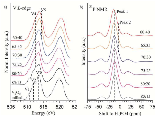
Fig. 2 a) V L-edge NEXAFS spectra of \text{V}_2\text{O}_5\text{:P}_2\text{O}_5 powders and milled \text{V}_2\text{O}_5 . b) ^{31}\text{P} MAS NMR of \text{V}_2\text{O}_5\text{:P}_2\text{O}_5 powders.
