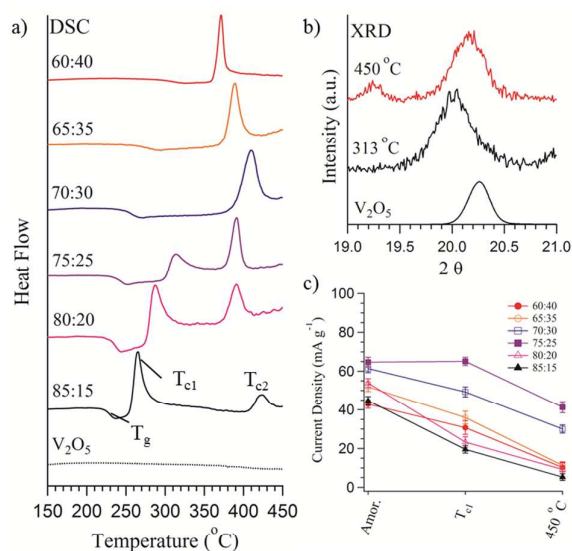
Figure 3. a) DSC scans of \text{V}_2\text{O}_5\text{:P}_2\text{O}_5 as-made powders and milled \text{V}_2\text{O}_5 . b) XRD patterns of 75:25 \text{V}_2\text{O}_5\text{:P}_2\text{O}_5 annealed at 313 °C and 450 °C. c) Current densities (mA/g) before and after annealing at T_{c1} and 450 °C.
