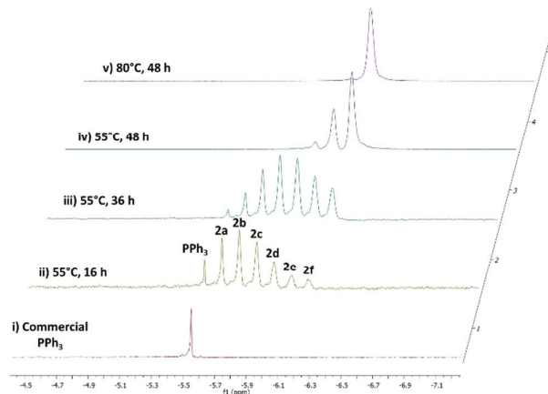
Fig. 2 Evolution of deuteration of \text{PPh}_3 ( 1 ) over time by ^{31}\text{P} -NMR.
