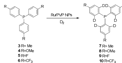
Scheme 2. Deuteration of para -substituted \text{PPh}_3 using Ru NPs.
