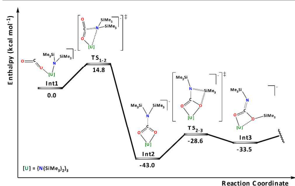
Figure 2. Part of the energy profile that leads to the formation of the isocyanate complex 2.
