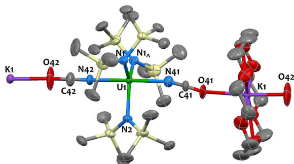
Figure 1. Solid-state molecular structure of [K(18c6)][U(N(SiMe_3)_2)_3(NCO)_2]_n 2 crystallized from THF/hexane. Hydrogen atoms and disorder are omitted for clarity. Uranium (green), potassium (purple), silicon (yellow), nitrogen (blue), oxygen (red) and carbon (grey) atoms are represented with 30% probability ellipsoids. Selected bond distances [Å] and angles [deg]: U1-N1 2.2679(2), U1-N2 2.2696(2), U1-O/N42 = 2.3358(1), U1-O/N41 = 2.3370(1), X42-C42-X'42 = 171.6(1), X41-C41-X'41 = 175.5(1).
