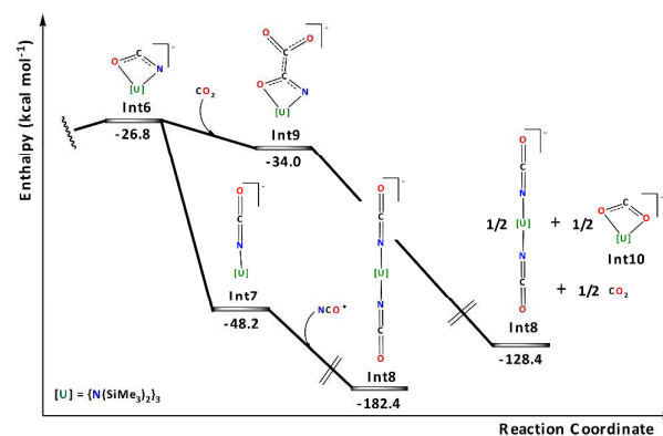
Figure 4. Part of the energy profile that leads to the formation of the isocyanate complex 2.
