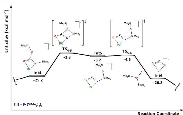
Figure 3. Part of the energy profile that leads to the formation of the isocyanate complex 2.
