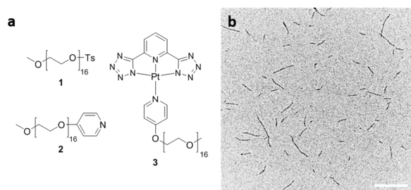
Fig. 1. (a) Structures of 1 , 2 , and 3 and (b) TEM image of polydisperse fibers formed by dissolving 3 in CHCl 3 at 0.5 mg/mL. Scale bar: 500 nm.
