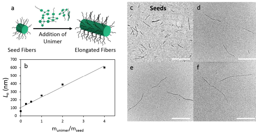
Fig. 2. (a) Schematic representation of the formation of elongated fibers. (b) Linear dependence of average contour length ( L_n ) on the unimer to seed mass ratio. (c) Seed micelles ( L_n = 60 nm, L_w/L_n = 1.14 ) formed through gentle sonication of polydisperse fibers (d-f) TEM micrographs of elongated fibers obtained by adding (d) 20 μg, (e) 40 μg, and (f) 80 μg of unimer (as a 2 mg/mL solution in hot MeCN) to 20 μg of seeds. Scale bars: 250 nm.
