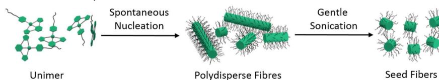
Scheme 1. Schematic representation of the formation of fibers from 3 . Dissolving the material in an OEG selective solvent produces a solution of polydisperse length cylinders; sonicating a solution of polydisperse fibers forms short seed fibres.
