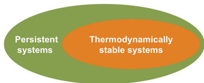
Figure 1: Diagram illustrating the set of thermodynamically stable systems as a sub-set of the more general set of persistent systems.
