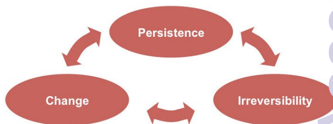
Figure 2: The Persistence Principle: 'Nature seeks persistent forms' expresses the idea of a logical relationship between persistence, change, and irreversibility. Changing things change, until they change into things that don't, thereby leading irreversibly to persistent forms.
