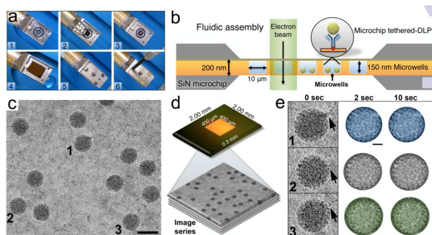
Fig. 2. Microfluidic system for in situ TEM imaging of virus particles. (a) The microfluidic chamber was assembled by placing O-ring fittings in the empty tip of the holder (steps 1 - 3). A flat chip was placed over top of the wet specimen chip (step 4) and the assembly was covered with a metal face-plate held in place by 3 brass screws (step 5 - 6). (b) Schematic of a cross-section through the fluidic chamber assembly positioned within the EM beam. Integrated microwells ( 10 \times 10 \mu\text{m} ) etched into the chip can each accommodate a solution layer of 150 nm thick. (c) Representative image of DLPs in liquid. (d) The base chip contained a transparent imaging window having array of microwells ( 400 \times 400 \mu\text{m} ). DLPs were tethered to the base chips and image series were recorded in the EM. (e) Representative DLPs (1 - 3) with viral mRNA transcripts (black arrows). Width of individual panels is \sim 120 \text{ nm} . Individual DLPs were contrast-inverted, masked by a diameter of \sim 80 \text{ nm} and colored for visualization purposes. Please see Movies S1 – S3, ESI ^\dagger .
