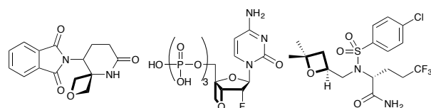
oxetano-thalidomide improved human blood plasma stability vs thalidomide 3',4'-oxetane nucleoside inhibitor of Hepatitis C virus (HCV NSSB; IC50 = 31 mM) γ-secretase inhibitor Pfizer Stepan et al.
