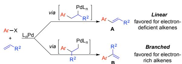
Scheme 1. Regioselectivity in Pd-catalyzed Heck coupling reactions.
