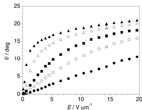
Fig 4. Electroclinic tilt angle \theta vs. electric field E measured in the SmA* phase formed by QL32-6 at T-T_{AC} = +0.2 K (▲), +0.8 K (△), +2 K (■), +3 K (○) and +5 K (●).
