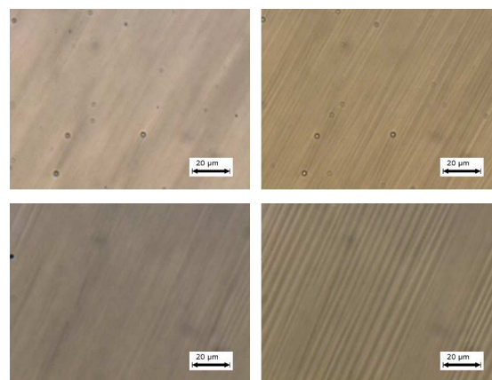
Fig 6. Polarized photomicrographs of QL32-6 (top) and 8422[2F3] (bottom) in 3 \mu\text{m} ITO glass cells with a rubbed nylon alignment substrate at T-T_{AC} = +0.2 K at zero-field (left) and with an applied 105 Hz square wave ac field of 7.3 \text{V } \mu\text{m}^{-1} ( QL32-6 ) and 3.7 \text{V } \mu\text{m}^{-1} ( 8422[2F3] ).
