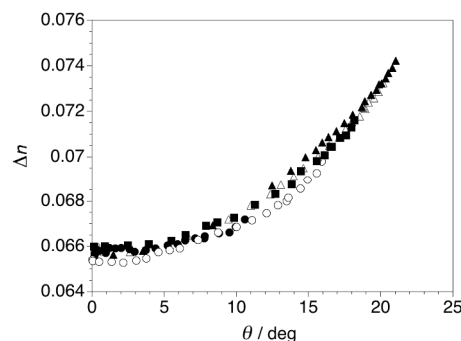
Fig 5. Birefringence \Delta n vs. electroclinic tilt angle \theta measured in the SmA* phase formed by QL32-6 at T-T_{AC} = +0.2 K (▲), +0.8 K (△), +2 K (■), +3 K (○) and +5 K (●).
