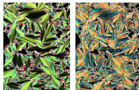
Fig 1. Polarized photomicrographs of QL32-6 at 63 °C in the SmA* phase (left) and at 61 °C in the SmC* phase (right).
