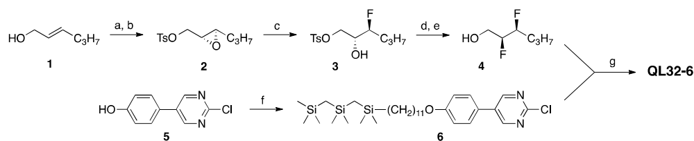
Scheme 1. Reagents and conditions: (a) (–)-diethyl D -tartrate, Ti(O i Pr) 4 , t -BuOOH, DCM; 22 (b) p -TsCl, pyridine, THF; (c) 70% HF•pyridine, DCM; (d) XtalFluor-E, Et 3 N•3HF, Et 3 N, DCM; 23 (e) Sml 2 , THF; 24 (f) 1-bromo-12,12,14,14,16,16-hexamethyl-12,14,16-trisilaheptadecane, Cs 2 CO 3 , acetone; (g) (i) 4 , NaH, THF, (ii) 6 .
