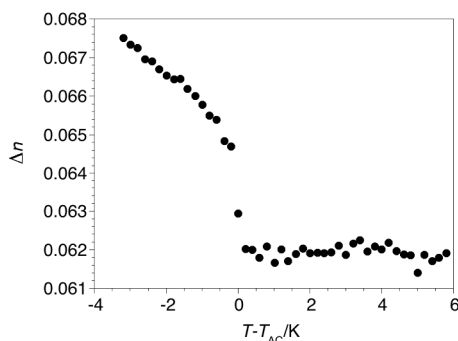
Fig 3. Birefringence \Delta n vs. reduced temperature T-T_{AC} for QL32-6 measured at zero-field.
