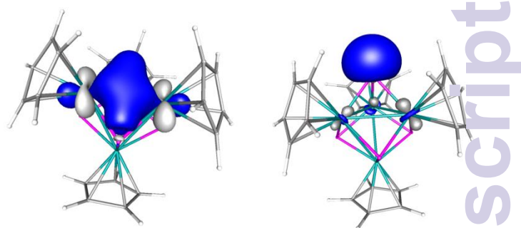
Fig. 2 Selected localized molecular orbitals representing the Mn–P bonding (left) and the lone pair of the phosphorus atoms (right) in [(\text{CpMn})_4(\text{P})_4] ( 1 ) in singlet spin state. Calculated at the BP86/def2-TZVP level of theory.
