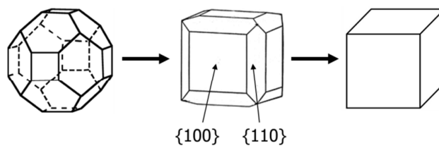
Figure 4 Growth of truncated rhombic dodecahedron particles to form cubic particles
