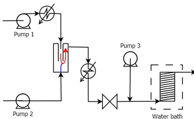
Figure 6 Schematic showing the combination of the synthesis and activation rigs where the ethanol used for activation is flown in at pump 3, after the back pressure regulator.
