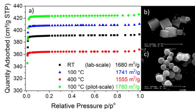
Figure 5 a) Nitrogen adsorption isotherms recorded for samples synthesised at RT, 100, and 400 °C using the lab-scale reactor and at 100 °C using the pilot-scale reactor. SEM pictures of ZIF-8 produced at 100 °C using b) the lab-scale reactor and c) the pilot-scale reactor are also shown.
