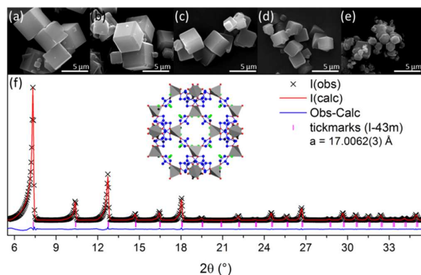
Figure 3 SEM data of ZIF-8 prepared using \text{NH}_4\text{OH} and synthesised at a \text{Zn}^{2+} concentration of 0.06 M and (a) room temperature, (b) 100 °C, (c) 200 °C, (d) 300 °C and (e) 400 °C. (f) Le Bail profile fit (I-43m) to XRD data of ZIF-8 prepared at 100 °C and 0.015 M ( \text{Zn}^{2+} )
