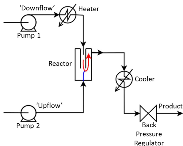
Figure 1 Schematic of continuous reactor used for the production of ZIF-8
