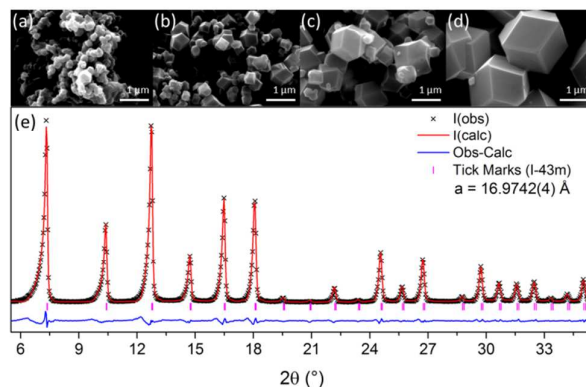
Figure 2 SEM data of ZIF-8 prepared using N(Et) 3 and synthesised at 100 °C and a Zn 2+ concentration of (a) 0.24 M, (b) 0.12 M, (c) 0.03 M and (d) 0.015 M. (e) Le Bail profile fit (l-43m) to XRD data of ZIF-8 prepared at 100 °C and 0.06 M (Zn 2+ )
