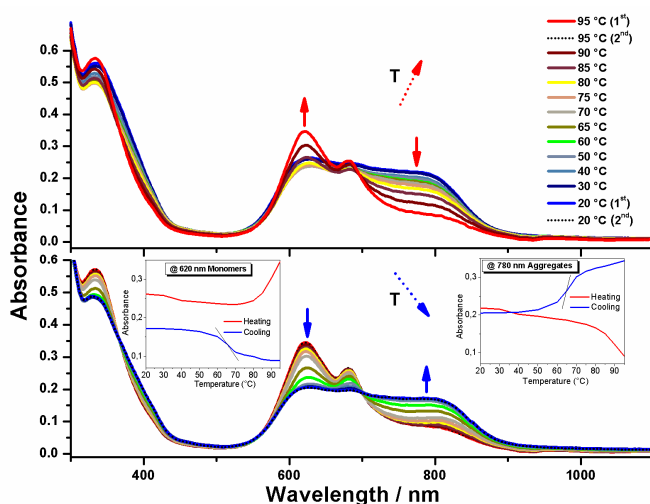
Fig. 3 Temperature-variable UV-Vis absorption of ZnPc-6d ( 3.3 \times 10^{-5} M) in dry n -heptane containing \sim 2 % dry dichloromethane. Above is the temperature-rise period and below is the temperature-fall period. The solid arrows reflect the electronic absorption's trend. Insets show the variable temperature evolution of the aggregate maxima monitored at 780 nm and that of the monomeric building blocks monitored at 620 nm. Black dotted traces show the almost perfect reversibility of the absorbance after a heating/cooling cycle.
