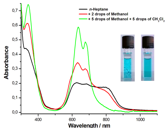
Fig. 2 Absorption spectra of ZnPc- 6d in dry n -heptane ( 3.3 \times 10^{-5} M, black line), after addition of two drops of methanol (red line) and followed by five more drops of methanol and five drops dichloromethane (the green line). A 3 mL cuvette with 1 cm pathlength is shown before (at left) and after addition of methanol and gentle shaking (at right). A microscopic image of the fluffs characteristic of these macro aggregates is provided in the Supporting Information (Fig. S7). Instead of methanol, pyridine or THF can be used to disassemble the aggregates (Fig. S9).
