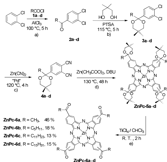
Scheme 1 Synthetic route of the desired tetraacylated ZnPc- 6a–d . Yields for procedures a) b) and c) performed several times on a multigram scale are detailed in the Supporting Information. The overall yields for ZnPc- 6a–d are based on the procedures d) and e) having 4a–d as starting material.
