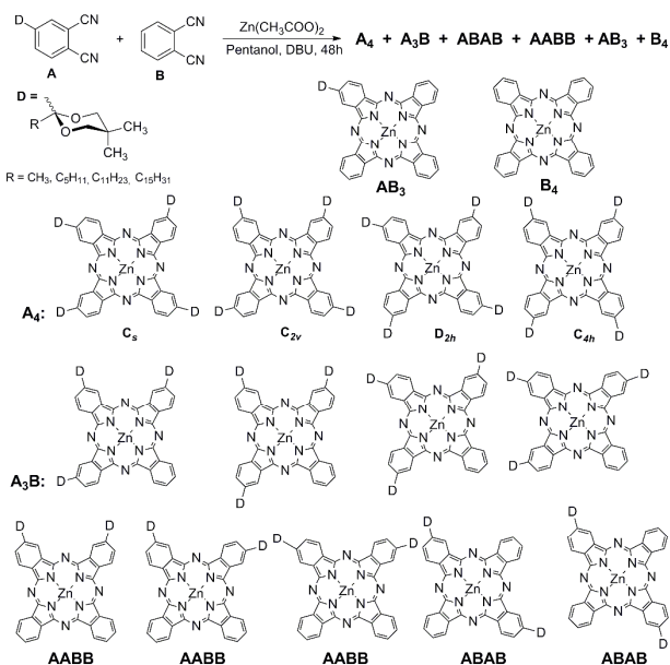
Scheme 2. Mixed condensation of two different phthalodinitriles A and B . D stands for the 1,3-dioxolane protecting group which after removal gives the acylated phthalocyanines with RC=O being either acetyl, hexanoyl, lauroyl or palmitoyl residues.
