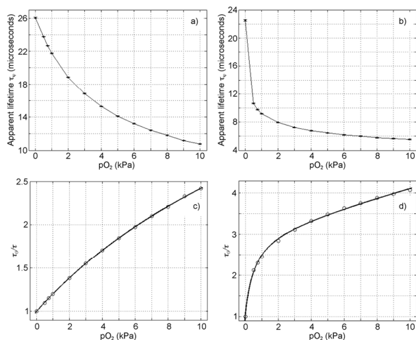
Fig. 4 Apparent lifetimes determined from the phase-shift ( \tau_0 in \mu\text{s} ) of a) 1-PS and b) 1-AP200/19 at 21 °C in the range 0-10 kPa \text{O}_2 ; and Stern-Volmer plot of c) 1-PS and d) 1-AP200/19 fitted using the Demas two-site model.
