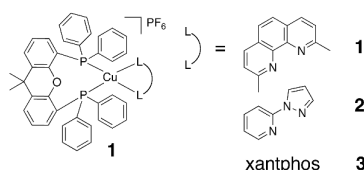
Fig. 1 Chemical structure of the Cu(I) complexes used in this work.
