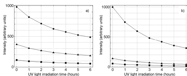
Fig. 5 Photostability of a) 1-PS and b) 1-AP200/19 at 21 °C for various oxygen concentrations using intensity measurements (● 0 kPa \text{pO}_2 ; ▲ 2 kPa \text{pO}_2 ; ■ 8 kPa \text{pO}_2 ).
