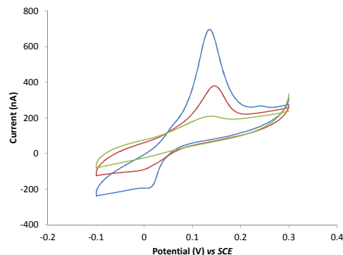
Figure 3. Consecutive cyclic voltammograms (blue) first, (red) second and (green) third cycle recorded at a working electrode consisting of BA-SAM with macrophage cells attached. The electrolyte was 50 mM PBS with 10% ethanol added as a toxin.
