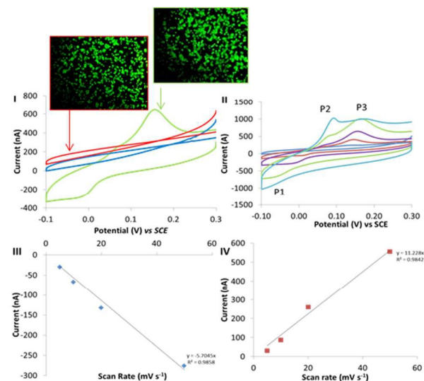
Figure 2. (I) Cyclic voltammograms recorded in 50 mM PBS at electrodes consisting of gold modified with COOH-SAM (red) and 3-aminophenylboronic acid in the presence of cells (green) and electrodes consisting of 3-aminophenylboronic acid which were not exposed to (blue) macrophage cells at 100 \text{ mV s}^{-1} . (II) Cyclic voltammograms recorded at scan rates of 5, 10, 20, 50, 100, \text{mV s}^{-1} in PBS on electrodes modified with 3-aminophenylboronic acid and cells. (III) Plots of reductive peak currents (P1) versus scan rate. (IV) Plots of oxidative peak currents (P3) at varying scan rates. Microscopy images of calcein stained cells adhered to COOH-SAM and BA-SAM obtained from modified surfaces exposed to cells for 3 hours confirming similar cell densities.
