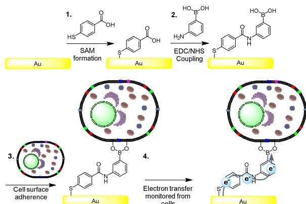
Figure 1. Schematic representation of (1) the formation of the carboxylic acid-terminated SAM, (2) the coupling of 3-aminophenylboronic acid and (3) the binding of cells via cyclic boronic ester formation. (4) Charge transfer events from cells enabled by the fabrication of electrodes with boronic acid (BA)-terminated self-assembled monolayers (SAMs).
