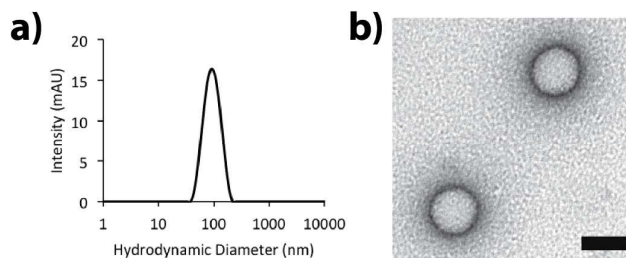
Figure 2: Characterization of P_{TBP} micelles show: (a) narrow distribution of 0.15 and diameter of 108 nm by DLS and (b) representative fields of view obtained by TEM (scale bar is 50 nm)
