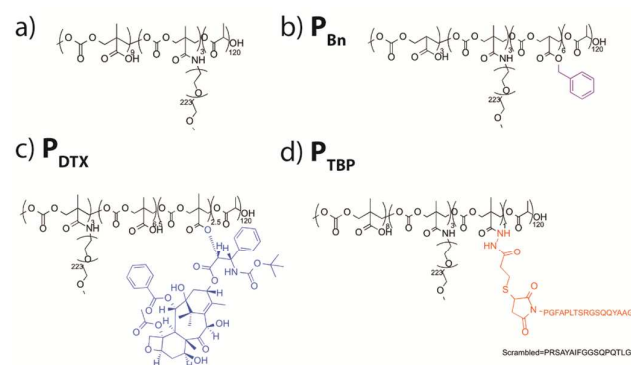
Figure 1. Hydrophobic backbone modifications of (a) P(LA-co-TMCC)-g-PEG with (b) benzyl groups ( P_{Bn} ), (c) docetaxel ( P_{DTX} ), and (d) taxol binding peptide ( P_{TBP} ) PGFAPLTSRGSQQYAA or the TBP scrambled control peptide ( P_{ScR} ) PRSAYAIFGGSQPTLQ.
