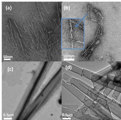
Fig. 2: TEM images of gels at (a) pH 6 (scale bar: 50nm) (b) pH 6.5 (scale bar: 100nm (Inset: zoomed image of twisted fibre)) (c) pH 7 (scale bar: 0.5μm) (d) pH 8 (scale bar: 0.5μm)
