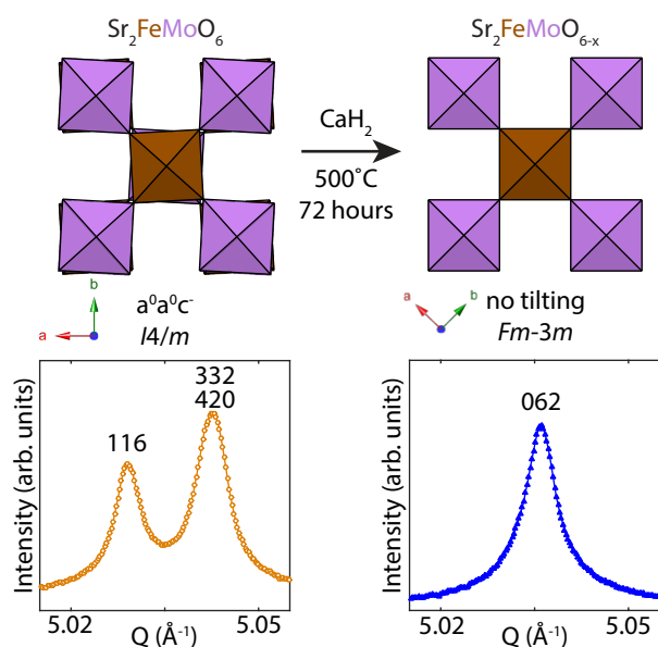
Fig. 1 Comparison of synchrotron XRD data of precursor (SFMO) and reduced (SFMO-red) materials. The reduction reaction eliminates the a^0a^0c^- octahedral tilting present in the starting material. A select region of the corresponding synchrotron XRD patterns are shown as the material transitions from tetragonal ( I4/m ; left) to cubic ( Fm\bar{3}m ; right). The Miller indices of the depicted peaks are included for reference. Complete diffraction patterns are provided in the ESI. †
