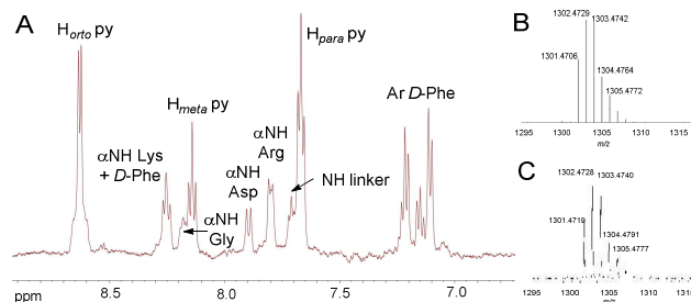
Fig. 3 1 H NMR spectra of conjugate 3 (A) in H 2 O/D 2 O 9:1, showing the region between 6.7 and 9.1 ppm. Expanded HR ESI mass spectrum of the molecular peak of 3 ([M+H] + ), calculated (B) and experimental (C).
