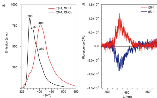
Fig. 3 a) Emission spectra of ( S )- 1 in MCH and CHCl 3 ( 5 \times 10^{-5} M, \lambda_{\text{exc}} = 297 nm; 298 K). b) CPL spectra of ( S )- 1 and ( R )- 1 in MCH ( 5 \times 10^{-5} M, \lambda_{\text{exc}} = 297 nm; 298 K).
