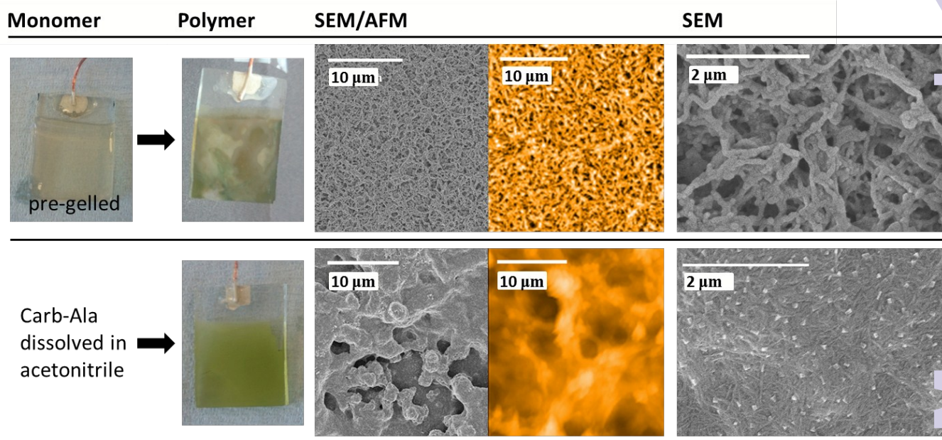
Figure 3. A comparison of the structures of large area polymer films grown on FTO glass electrodes. The top row shows the structure of the polymer formed when a gel is electropolymerized. The film grown from the pre-formed gel has a slight brown discoloration due to remaining hydroquinone/quinone within the polymer. The bottom row shows films obtained from the direct electropolymerization of Carb-Ala dissolved in acetonitrile. In both cases, the AFM (films grown from 2 mgmL -1 Carb-Ala) and SEM (films grown from 2.5 mgmL -1 Carb-Ala) images underline the large differences in the microstructures of polymer grown via the gel phase.
