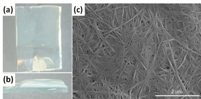
Figure 1. Photographs of a transparent Carb-Ala gel formed on an ITO-coated glass slide from (a) the top and (b) the side. (c) shows a SEM image of the xerogel formed by drying the gel in air.
