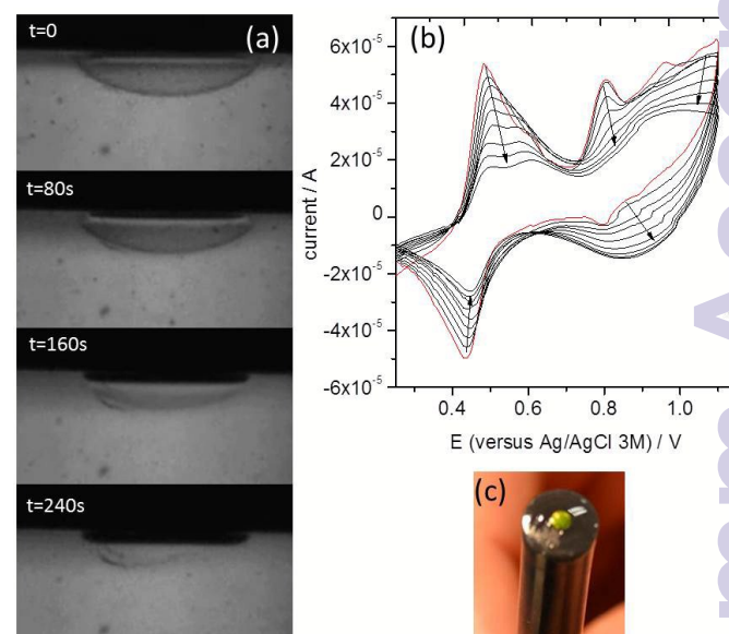
Figure 2. (a) In-situ polymerization of a pre formed gel on the surface of a gold disc electrode. At t=0 , the gel is visible as a transparent hemi-sphere above the electrode surface. As the electrode was cycled above the oxidation potential for the monomer, the gel collapsed into a denser polymer layer on the electrode surface. The stills show the progression during the first 8 CVs at 50 mVs -1 (34 seconds per scan). The surface attached polymer was electrochromic and cycled between green and colorless during successive scans. (b) Cyclic voltammograms taken during the polymerization of the gel shown in part (a). The peaks at 0.75 V are connected with the oxidation and reduction of the Carb-Ala monomer/polymer. The arrows show the evolution of the peaks with time. (c) photograph showing the green polymer grown on the gold disc electrode
