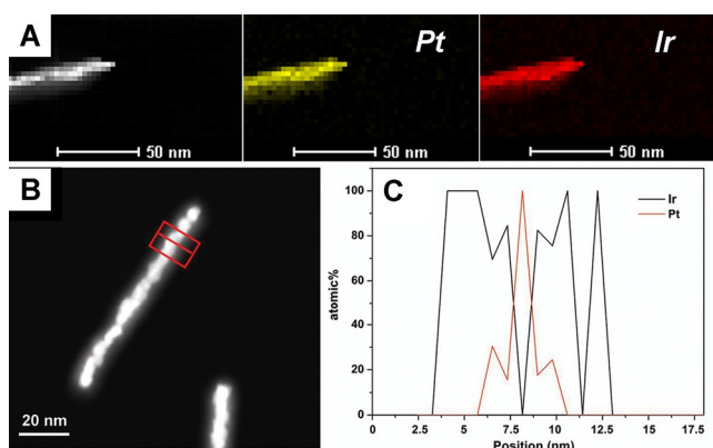
Figure 2. (A) Elemental mapping for the Pt@Ir nanocomplexes; (B) HAADF image of the Pt@Ir nanocomplexes; (C) Cross-sectional elemental composition of the marked area in (B).
