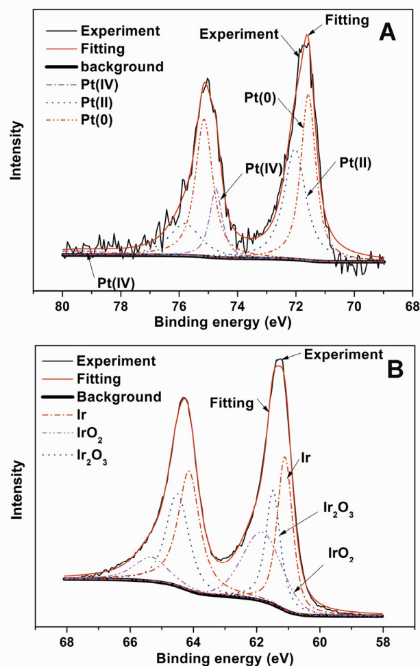
Figure 3. High resolution XPS spectra and fitting of the (A) Pt 4f and (B) Ir 4f spectral regions for the Ir@Pt nanocomplexes.
