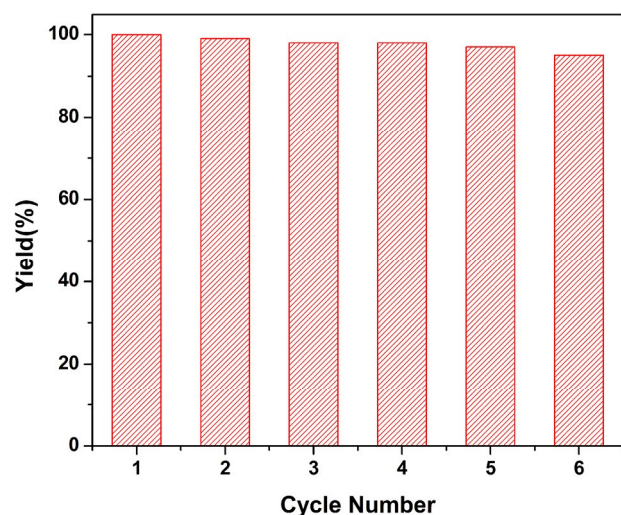
Figure 4. The catalytic stability of Pt@Ir nanocomplexes in the hydrogenation of nitrobenzene in different cycles.
