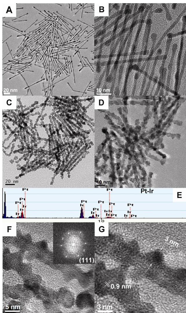
Figure 1. TEM and HRTEM images of the Pt (A, B) and Pt@Ir (C, D) nanocomplexes; EDS analysis of the Pt@Ir nanocomplexes (E); HRTEM images and selected area electron diffraction pattern of the Pt@Ir nanocomplexes (F, G).
