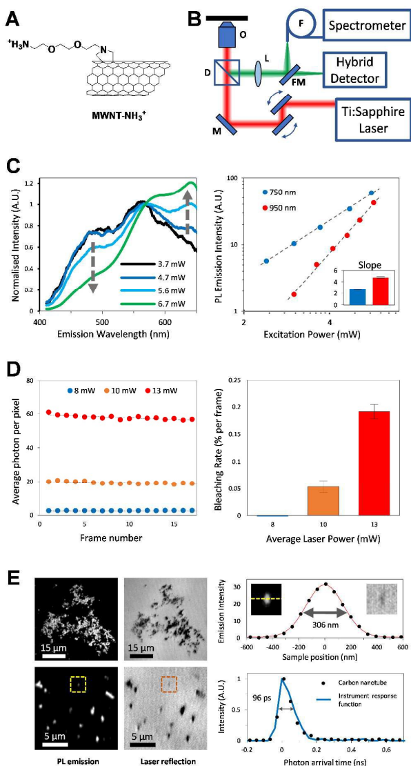
Figure 1. Optical properties of MWNT-NH 3 + derivative. (A) Diagram showing the structure of the MWNT-NH 3 + derivative investigated in this work. (B) Schematic representation of the multiphoton microscope used in this study. (C) Left panel: multiphoton photoluminescence spectra of drop-casted MWNT-NH 3 + at 750 nm excitation using different laser powers. Photoluminescence signals were normalized to 568 nm emission intensities. Right panel: log-log plot of the photoluminescence intensity as a function of the laser power at both 750 nm and 950 nm excitation wavelengths. Slope
