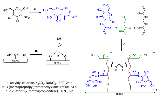
Scheme 1 Synthetic route to glass-bound glycopolymer hydrogels.
