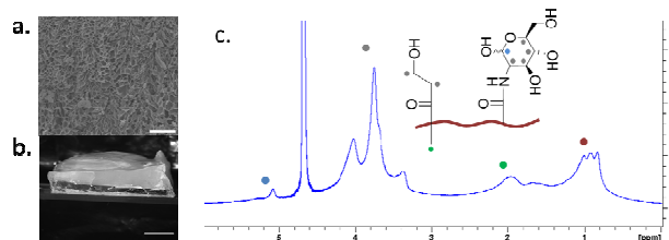
Figure 1 a. Glass-bound hydrogel's internal structure by SEM (scale: 100 μm) and b. the whole sample (scale: 5 mm); c. HR-MAS 1 H NMR spectrum of a 30 mol% AGA hydrogel.
