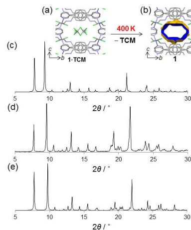
Fig. 4 Crystal structure of the host framework 1 obtained by in situ heating 1\cdot\text{TCM} to 400 K (a,b). Simulated XRPD pattern of 1 at 400 K (c). Experimental XRPD pattern obtained by rapid mixing a TCM solution of L and \text{ZnCl}_2 (MeOH) at 300 K (d); and simulated from single crystal X-ray diffraction (100 K) 1\cdot\text{TCM} (e). Colour code as in Fig. 1.
