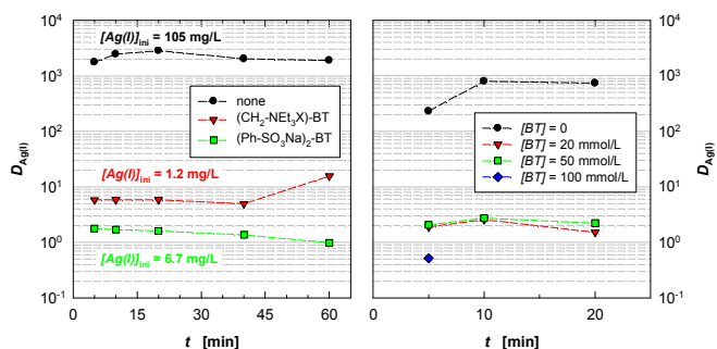
Figure 4. Influence of masking agents 10 and 13 on the extraction of Ag(I) into CyMe 4 -BTBP 1 . Organic phase: 10 mM CyMe 4 -BTBP 1 + 5 mM TODGA in 1-octanol. Aqueous phase: Ni(II), Pd(II), Ag(I), Cd(II) (1 mM each) with or without 20 mM masking agent 10 or 13 (left), or with varied concentrations of 13 (right) in 2 M HNO 3 . T = 20 °C, A/O = 1 ((CH 2 NEt 3 X) 2 -BT = ligand 13 , (PhSO 3 Na) 2 -BT = ligand 10 ).
