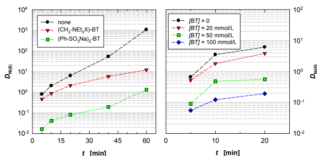
Figure 2. Influence of masking agents 10 and 13 on the extraction of Ni(II) into CyMe 4 -BTBP 1 . Organic phase: 10 mM CyMe 4 -BTBP 1 + 5 mM TODGA in 1-octanol. Aqueous phase: Ni(II), Pd(II), Ag(I), Cd(II) (1 mM each) with or without 20 mM masking agent 10 or 13 (left), or with varied concentrations of 13 (right) in 2 M HNO 3 . T = 20 °C, A/O = 1 ((CH 2 NEt 3 X) 2 -BT = ligand 13 , (PhSO 3 Na) 2 -BT = ligand 10 ).
