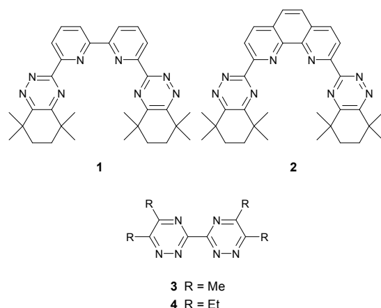
Figure 1. Structures of CyMe 4 -BTBP 1 , CyMe 4 -BTPhen 2 and 3,3'-bis(1,2,4-triazine) ligands 3 and 4 .
