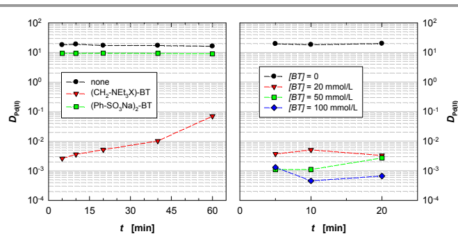
Figure 3. Influence of masking agents 10 and 13 on the extraction of Pd(II) into CyMe 4 -BTBP 1 . Organic phase: 10 mM CyMe 4 -BTBP 1 + 5 mM TODGA in 1-octanol. Aqueous phase: Ni(II), Pd(II), Ag(I), Cd(II) (1 mM each) with or without 20 mM masking agent 10 or 13 (left), or with varied concentrations of 13 (right) in 2 M HNO 3 . T = 20 °C, A/O = 1 ((CH 2 NEt 3 X) 2 -BT = ligand 13 , (PhSO 3 Na) 2 -BT = ligand 10 ).
