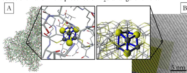
Figure 1. Schematic representation of (a) the ferredoxin center of the CO dehydrogenase enzyme, 11f (b) the greigite surface, Fe 3 S 4 (001), showing enhanced the cubane structure.
