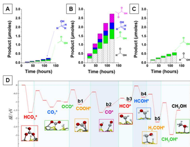
Figure 3. Formation of formic acid, acetic acid, methanol and pyruvic acid at (a) pH= 4.5; (b) pH= 6.5; (c) pH= 10.5. (d) Potential energy profile for the mechanism of \text{HCO}_3^- reduction to \text{CH}_3\text{OH} , on the \text{Fe}_3\text{S}_4 (111).
