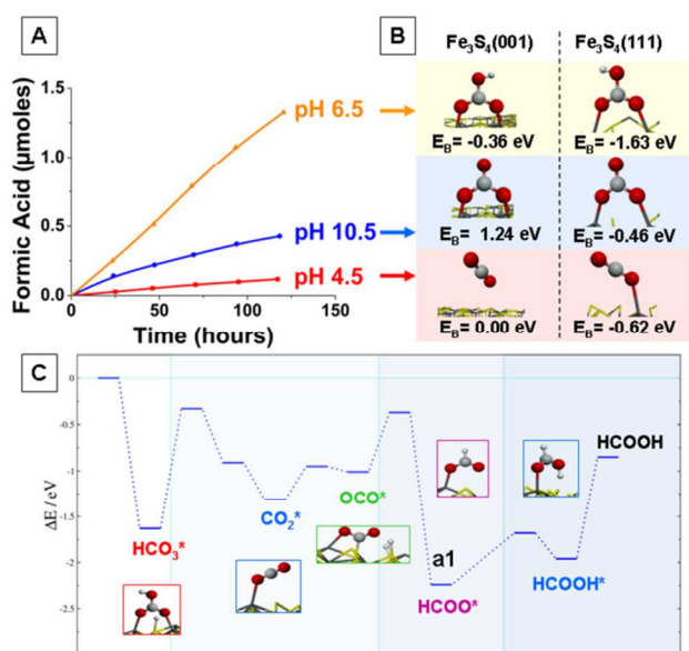
Figure 2. (a) Formic acid formation as a function of time under different pH conditions; (b) Representation of reactants on both the (001) and (111) surfaces as a function of the solution pH, binding energies ( E_B ) provided as inset; (c) Potential energy surface for the mechanism of \text{HCO}_3^- reduction to \text{HCOOH} on the \text{Fe}_3\text{S}_4 (111). Adsorbed intermediate species are denoted by * and their proposed structures are shown as insets in the figure.
