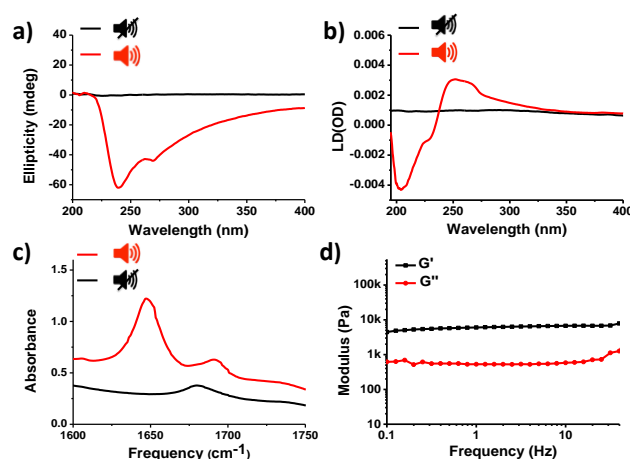
Fig. 2 (a) CD, (b) LD and (c) FT-IR spectra of ^D FFD in methanol before and after ultrasound irradiation. (d) Rheology of the elastic modulus ( G' ) and viscous modulus ( G'' ) of ^D FFD organogel after ultrasound irradiation. The concentration is 25 mM.
