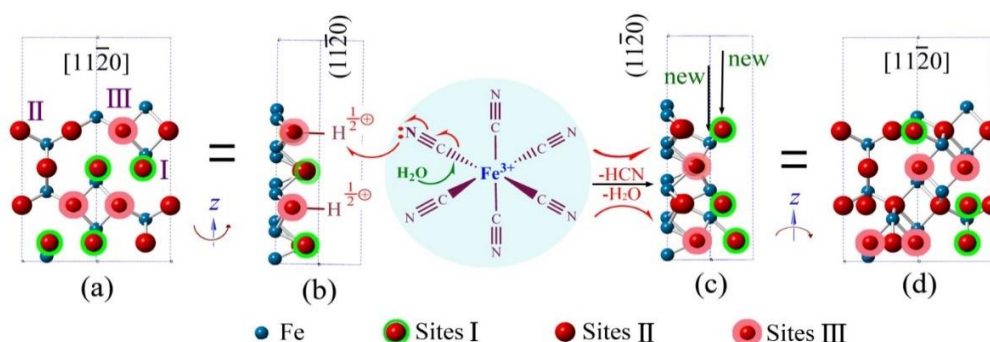
Fig. 2 Schematic drawing of surface adsorption of a [\text{Fe}(\text{CN})_6]^{3-} anion to the positively charged triply coordinated hydroxyl group on the \{11\bar{2}0\} surface and its surface hydrolysis into \alpha\text{-Fe}_2\text{O}_3 . (a), (b) Top view and profile view with H on sites III of the \{11\bar{2}0\} surface. (c), (d) Profile view and top view of the surface with a newly deposited layer of \alpha\text{-Fe}_2\text{O}_3 .
