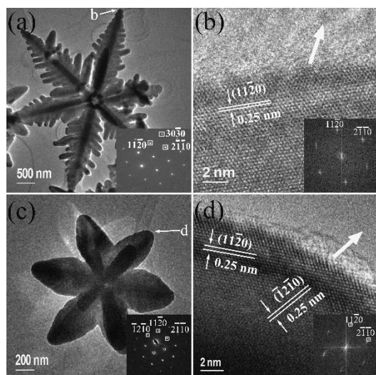
Fig. 3 (a) TEM image of a typical 'starfish' particle from the sample prepared with 0.12 mol/L octylamine. The inset is the corresponding SAED pattern. (b) HRTEM image of a tip area, marked by 'b', of the particle in (a). (c) TEM image of a 'flower' \alpha -Fe 2 O 3 particle from the sample prepared with 0.24 mol/L octylamine. The inset is the corresponding SAED pattern. (d) HRTEM image from a tip area, marked by 'd', of the particle in (c). The insets in (b) and (d) are the FFT pattern from the whole areas. The arrows in (b) and (d) indicate the crystal growth directions of [10\bar{1}0] .
