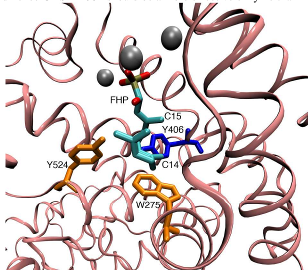
Figure 2. Homology model of GDS with farnesyl hydroxyphosphonate (FHP) bound at the active site based on the known structure of 5- epi -aristolochene synthase from Nicotiana tabacum coordinated to the inhibitor FHP (PDB-5EAT). 22 Active site residues Y406 (blue), Y524 and W275 (orange) that were targeted for site directed mutagenesis are shown along with three Mg 2+ -cofactor ions (silver spheres).
