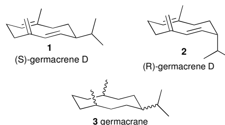
Figure 1. Enantiomers of germacrene D, ( S )-germacrene D (1), ( R )-germacrene D (2) and germacrane (3).
