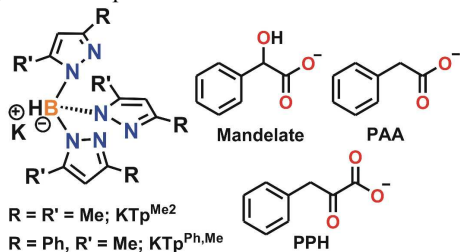
Fig. 1 Ligands and model substrates.
