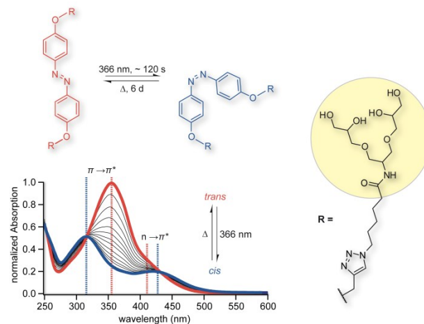
Fig. 1 UV/VIS absorption spectra showing the trans to cis conversion of GlazoG1 6 . The photoinduced isomerization is completed after 120 s, whereas the thermal cis to trans conversion takes 6 d when stored in the dark. The side chains of GlazoG1 6 are abbreviated by an "R".
