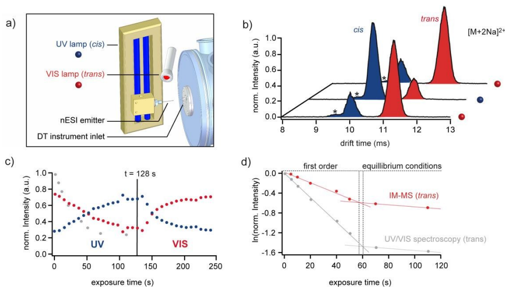
Fig. 2 Ion mobility-mass spectrometry (IM-MS) of G1azoG1 6 . a) Modified source region of the utilized DT IM-MS instrument. b) Arrival time distributions (ATDs) of [M+2Na]^{2+} ions after irradiation at \lambda = 366 nm (blue dot) or with visible light (red dot), respectively. Peaks resulting from neighbouring masses are labelled with an asterisk. c) Relative intensities of the cis - and trans populations plotted against exposure time. The normalized intensity of trans G1azoG1 6 observed via UV/VIS spectroscopy is shown as grey circles for comparison. d) Logarithmic plot of the normalized intensity of trans G1azoG1 6 at 366 nm as a function of exposure time determined by IM-MS (red circles) and UV/VIS spectroscopy (grey circles).
