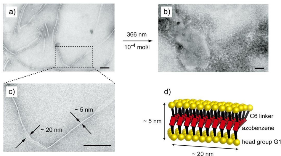
Fig. 3 Aggregates of GlazoG1 6 visualized by transmission electron microscopy (TEM). a) Twisted tapes formed by trans GlazoG1 6 with widths around 20 nm and a constant thickness of 5 nm. b) Amorphous structures formed by cis GlazoG1 6 ( 10^{-4} M) upon UV irradiation. c) Twisted tape formed by trans GlazoG1 6 ( 10^{-4} M). d) Schematic model of trans GlazoG1 6 describing the twist along the longitudinal axis of the tapes. The black scale bars are indicating 100 nm.
