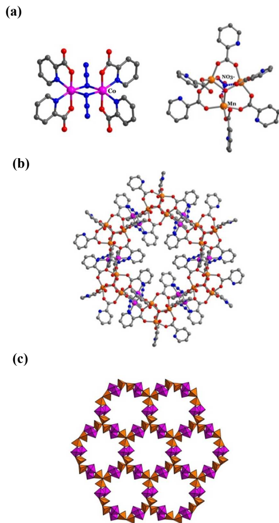
Fig 1. (a) Ball and stick view of the [Co 2 (pic) 4 (N 3 ) 2 ] 2- and [Mn 3 O(pic) 6 (NO 3 ) 3 ] 3- units in 1 ; (b) View of triacontanuclear heterometallic [Co 2 (Mn 3 O)(pic) 6 (NO 3 ) 6 ] 6 wheel motif observed in 1 with a dimension of 3.2 × 0.8 nm and an hydrophobic inner diameter of 0.6 nm; (c) Polyhedral-type view of the hexagonal network of [Co 2 Mn 2 ] 6 icositetranuclear rings. The Co and Mn polyhedra are shown in purple and brown colors, respectively. Color code: Co purple, Mn orange, Na dark green, O red, N blue, C grey. Hydrogen atoms have been omitted for clarity.
