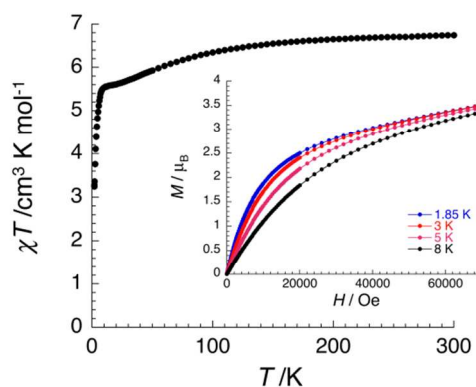
Fig 2. Temperature dependence of \chi T product at 1000 Oe (where \chi is the molar magnetic susceptibility equal to the ratio between the magnetization and the applied magnetic field, M/H , per mole of {CoMn} pair) between 1.85 and 300 K for a polycrystalline sample of 1 . Inset: M vs H plot for 1 between 1.85 and 8 K at magnetic fields between 0 and 7 T with sweep-rates of 100 – 200 Oe/min. The solid line is a guide for eyes.
