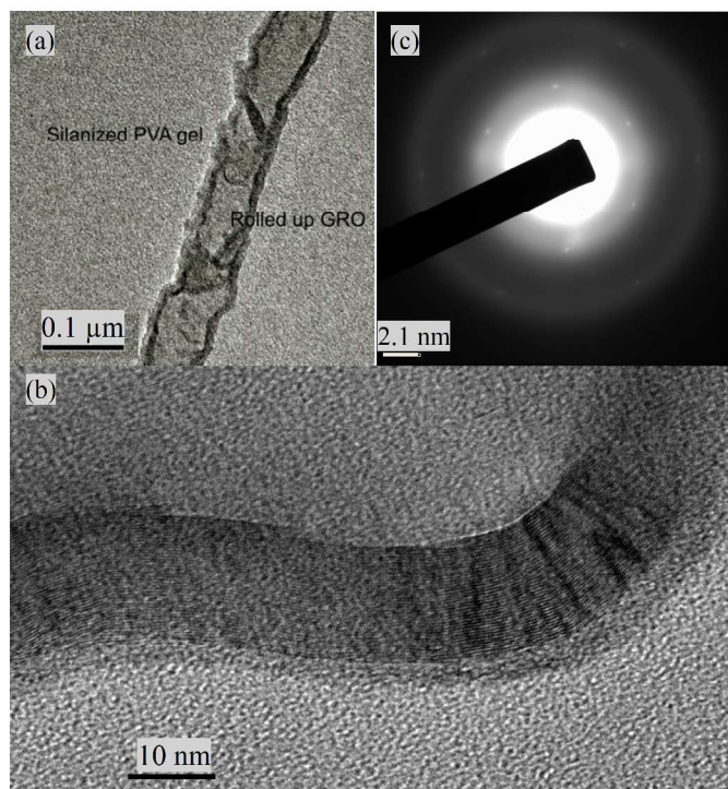
Figure 2: (a) TEM image of a 'rolled up' graphene oxide wire in the silanized PVA-GO (Si) gels (b) High resolution TEM (HRTEM) and (c) selected-area electron diffraction pattern images.
