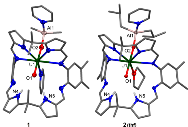
Figure 1 Solid-state structures of 1 and 2(thf) , front view. For clarity, all hydrogen atoms except the pyrrole NHs and all solvent molecules are omitted (displacement ellipsoids are drawn at 50% probability). Selected bond lengths (Å) for 1 : U1-O1 1.857(3), U1-O2 1.962(3), O1-N4 2.964(5), O1-N5 3.068(5). O1-U1-O2 174.3(1)°; 2 : U1-O1 1.855(2), U1-O2 1.962(2), O1-N4 3.033(4), O1-N5 3.027(4). O1-U1-O2 175.1(1)°.
