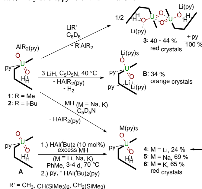
Scheme 2 Transmetalation reactions of 1 and 2 with R' i Li, LiH, NaH and KH, and the HAl( i -Bu) 2 - catalyzed reduction of [U VI O 2 (H 2 L)] by MH.
