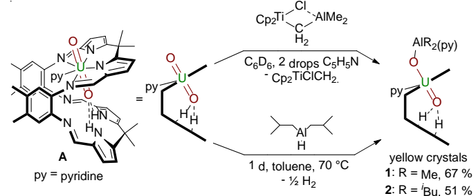
Scheme 1 Reductive aluminations of [(UO 2 )(py)(H 2 L)], A by Tebbe's reagent or DIBAL
