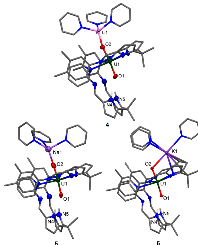
Figure 3 Solid-state structures of 4 , 5 and 6 (side view). For clarity, all hydrogen atoms except pyrrole NHs and all solvent molecules are omitted (displacement ellipsoids are drawn at 50% probability). Selected bond lengths (Å) for 4 : U1-O1 1.853(6), U1-O2 1.884(7), O1-N4 3.09(1), O1-N5 3.10(1). O1-U1-O2 173.8(3)°; 5 : U1-O1 1.844(5), U1-O2 1.856(7), O1-N4 3.010(9), O1-N5 2.988(8). O1-U1-O2 174.2(3)°; 6 : U1-O1 1.871(2), U1-O2 1.837(2), O1-N4 2.898(4), O1-N5 2.932(4). O1-U1-O2 176.1(1)°.
