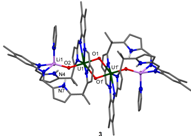
Figure 2 Solid-state structure of 3 . For clarity, all hydrogen atoms except pyrrole NH and all solvent molecules are omitted (displacement ellipsoids are drawn at 50% probability). Selected bond lengths (Å): U1-O1 1.908(2), U1-O2 1.891(2), U1-O1' 2.372(3), N4-O2 3.269(4), N7-O2 3.198(5). O1-U1-O2 177.7(1)°. U1...U1': 3.5199(9) Å.
