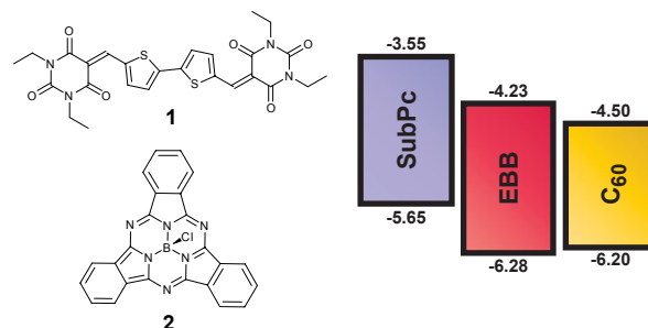
Fig. 1: Chemical structures of EBB 1 and SubPc 2 and corresponding energy levels including C 60 .
