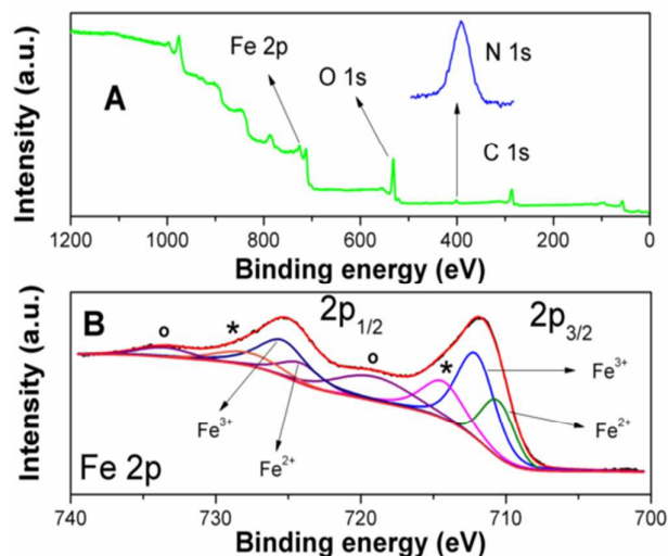
Figure 2. A) XPS spectra of \text{Fe}_3\text{O}_4 @pDA MNPs; inset: expanded spectrum of the N1s core line. B) Deconvoluted high-resolution XPS spectra for Fe 2p_{3/2} and Fe 2p_{1/2} core-level lines for \text{Fe}_3\text{O}_4 @pDA MNPs; (o) \text{Fe}^{3+} shake-up satellites and (*) \text{Fe}^{2+} shake-up satellites.
