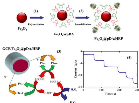
Scheme 1. Schematic illustration of the preparation of core-shell \text{Fe}_3\text{O}_4 @pDA/HRP nanoparticles (1 and 2) and the \text{Fe}_3\text{O}_4 @pDA/HRP-GCE biosensor (3) as well as the amperometric responses obtained for successive additions of 125 \mu\text{L} of 3 mM HQ (4).
