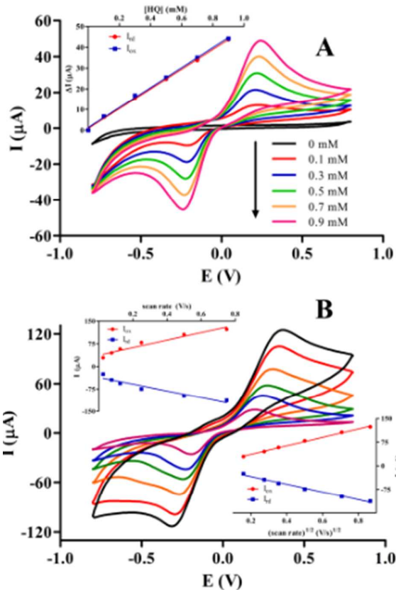
Figure 5. (A) CVs recorded at a GCE/Fe 3 O 4 @pDA/HRP biosensor in PBS solution, pH 7.4 containing different HQ concentrations (scan rate: 100 mV s -1 ); inset: linear dependence between HQ concentration and the anodic ( I_{ox} ) and cathodic ( I_{rd} ) peak current values. (B) CVs recorded at a GCE/Fe 3 O 4 @pDA/HRP biosensor in PBS containing 1 mM HQ at different scan rates; insets: dependence of the anodic and cathodic peak current values with the scan rate and the square-root of the scan rate.
