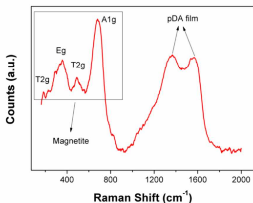
Figure 3. Raman spectrum of \text{Fe}_3\text{O}_4 @PDA MNPs.
