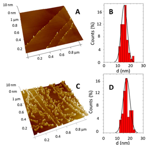
Figure 1. Typical 1 \times 1 \mu\text{m}^2 AFM images (A, C) and histograms showing particle-size distribution (B, D) for \text{Fe}_3\text{O}_4 (A, B) and \text{Fe}_3\text{O}_4 @pDA MNPs (C, D).
